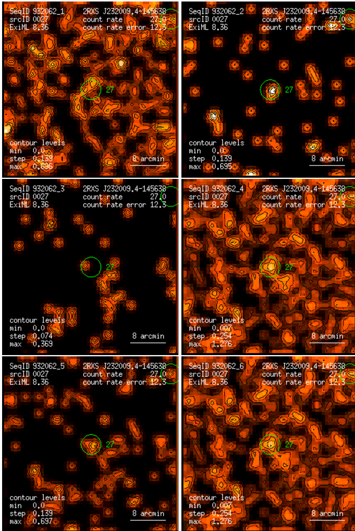
Figure 27: RASS 932062: detection 0027: band rate images, Gaussian filter: (1) PSPC channels 11 – 41, (2) 52 – 90, (3) 91 – 201, (4) 11 – 235, (5) 52 – 201, (6) 11 – 201. Broad band rates in counts/ks. Band rate contour levels in counts/ks/arcmin 2 .
