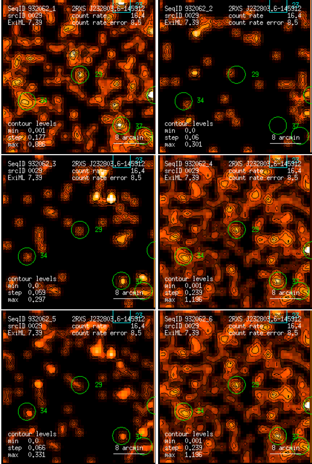
Figure 29: RASS 932062: detection 0029: band rate images, Gaussian filter: (1) PSPC channels 11 – 41, (2) 52 – 90, (3) 91 – 201, (4) 11 – 235, (5) 52 – 201, (6) 11 – 201. Broad band rates in counts/ks. Band rate contour levels in counts/ks/arcmin 2 .
