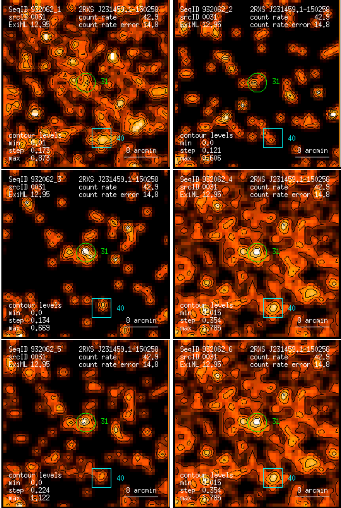
Figure 31: RASS 932062: detection 0031: band rate images, Gaussian filter: (1) PSPC channels 11 – 41, (2) 52 – 90, (3) 91 – 201, (4) 11 – 235, (5) 52 – 201, (6) 11 – 201. Broad band rates in counts/ks. Band rate contour levels in counts/ks/arcmin 2 .
