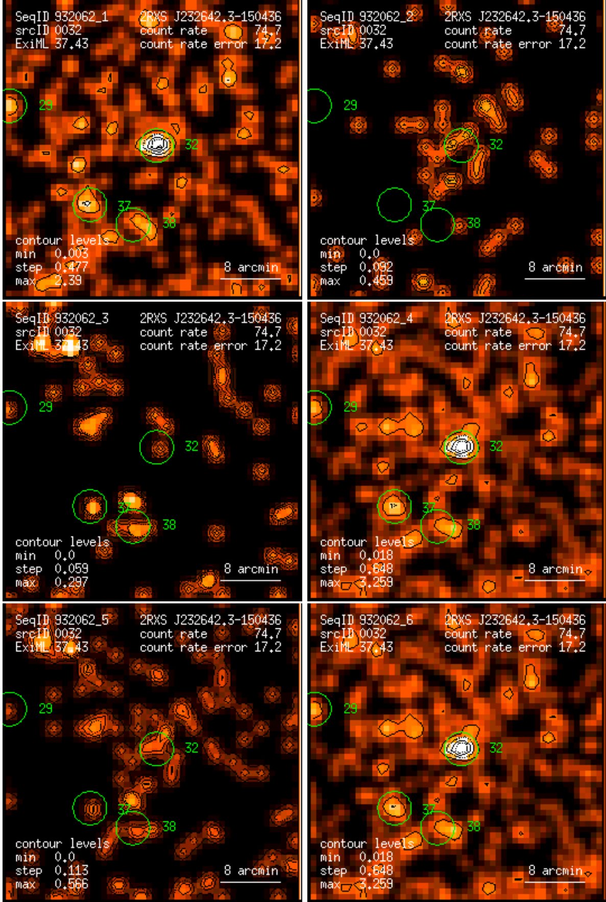
Figure 32: RASS 932062: detection 0032: band rate images, Gaussian filter: (1) PSPC channels 11 – 41, (2) 52 – 90, (3) 91 – 201, (4) 11 – 235, (5) 52 – 201, (6) 11 – 201. Broad band rates in counts/ks. Band rate contour levels in counts/ks/arcmin 2 .
