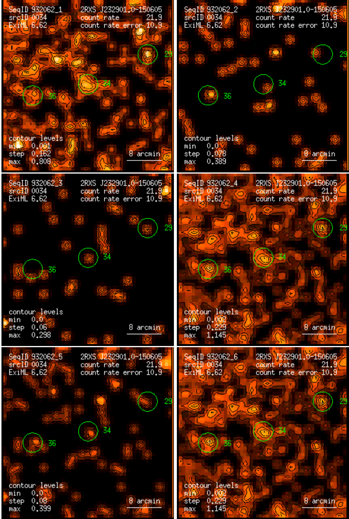
Figure 34: RASS 932062: detection 0034: band rate images, Gaussian filter: (1) PSPC channels 11 – 41, (2) 52 – 90, (3) 91 – 201, (4) 11 – 235, (5) 52 – 201, (6) 11 – 201. Broad band rates in counts/ks. Band rate contour levels in counts/ks/arcmin 2 .
