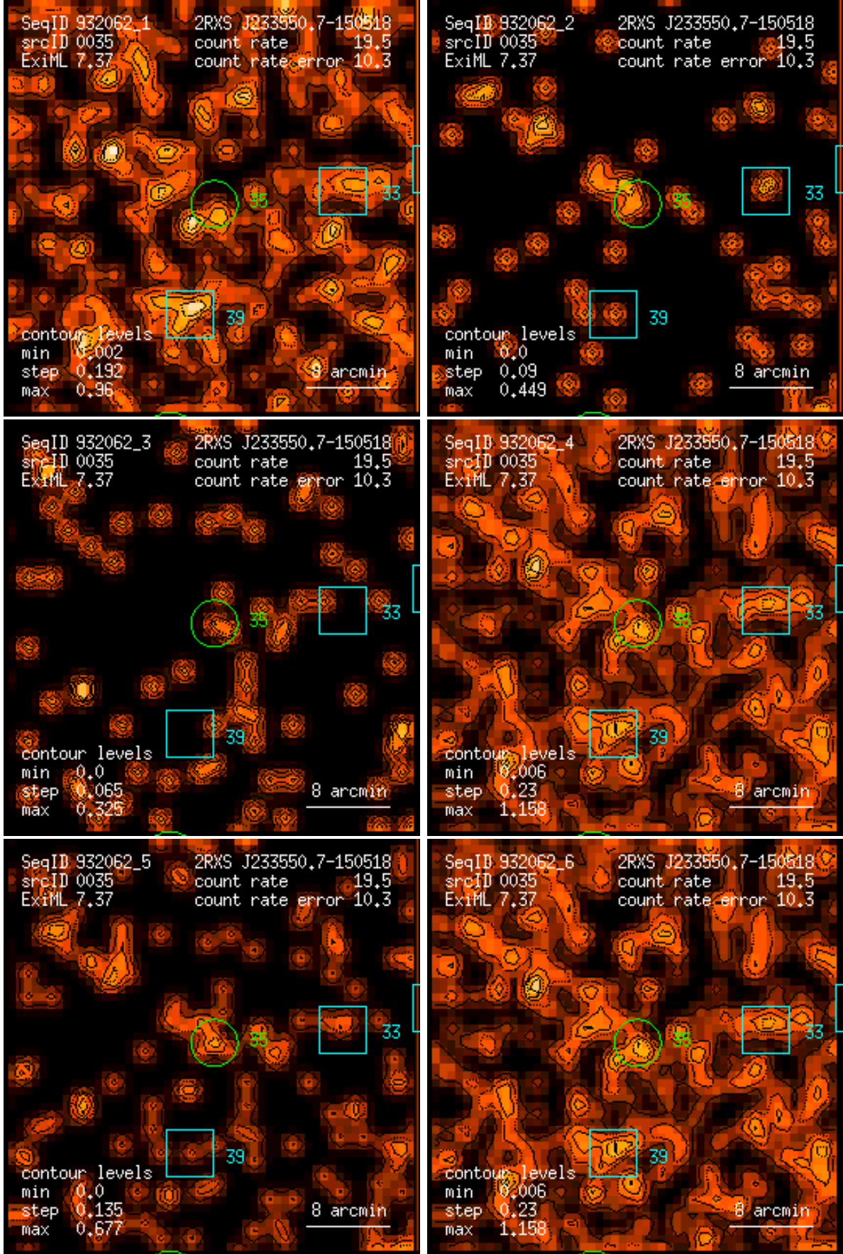
Figure 35: RASS 932062: detection 0035: band rate images, Gaussian filter: (1) PSPC channels 11 – 41, (2) 52 – 90, (3) 91 – 201, (4) 11 – 235, (5) 52 – 201, (6) 11 – 201. Broad band rates in counts/ks. Band rate contour levels in counts/ks/arcmin 2 .
