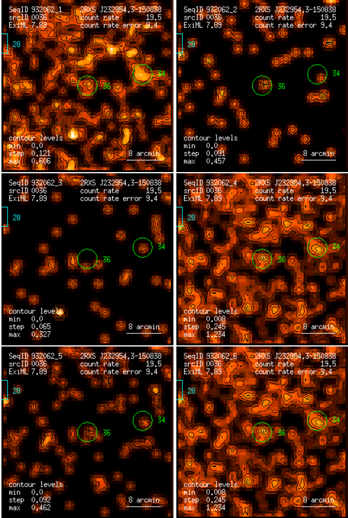
Figure 36: RASS 932062: detection 0036: band rate images, Gaussian filter: (1) PSPC channels 11 – 41, (2) 52 – 90, (3) 91 – 201, (4) 11 – 235, (5) 52 – 201, (6) 11 – 201. Broad band rates in counts/ks. Band rate contour levels in counts/ks/arcmin 2 .
