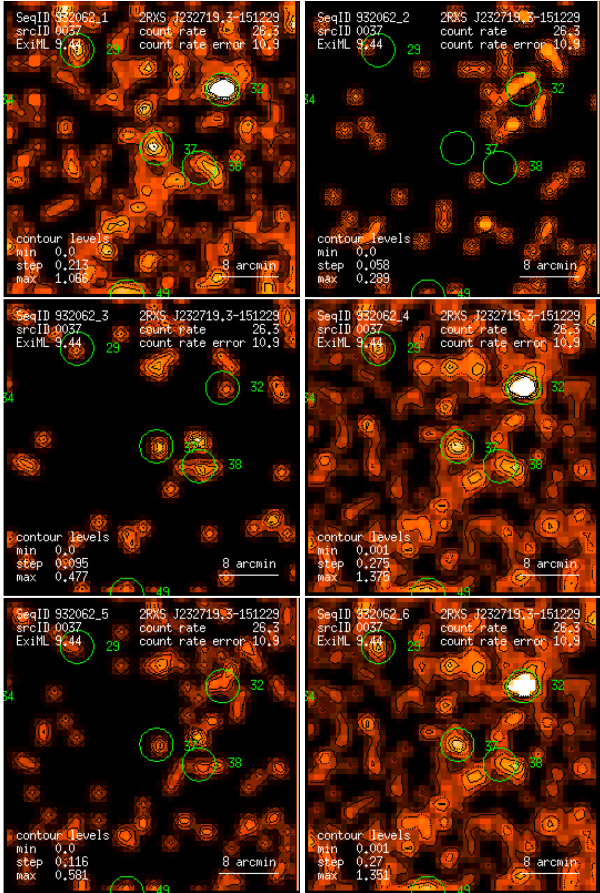
Figure 37: RASS 932062: detection 0037: band rate images, Gaussian filter: (1) PSPC channels 11 – 41, (2) 52 – 90, (3) 91 – 201, (4) 11 – 235, (5) 52 – 201, (6) 11 – 201. Broad band rates in counts/ks. Band rate contour levels in counts/ks/arcmin 2 .
