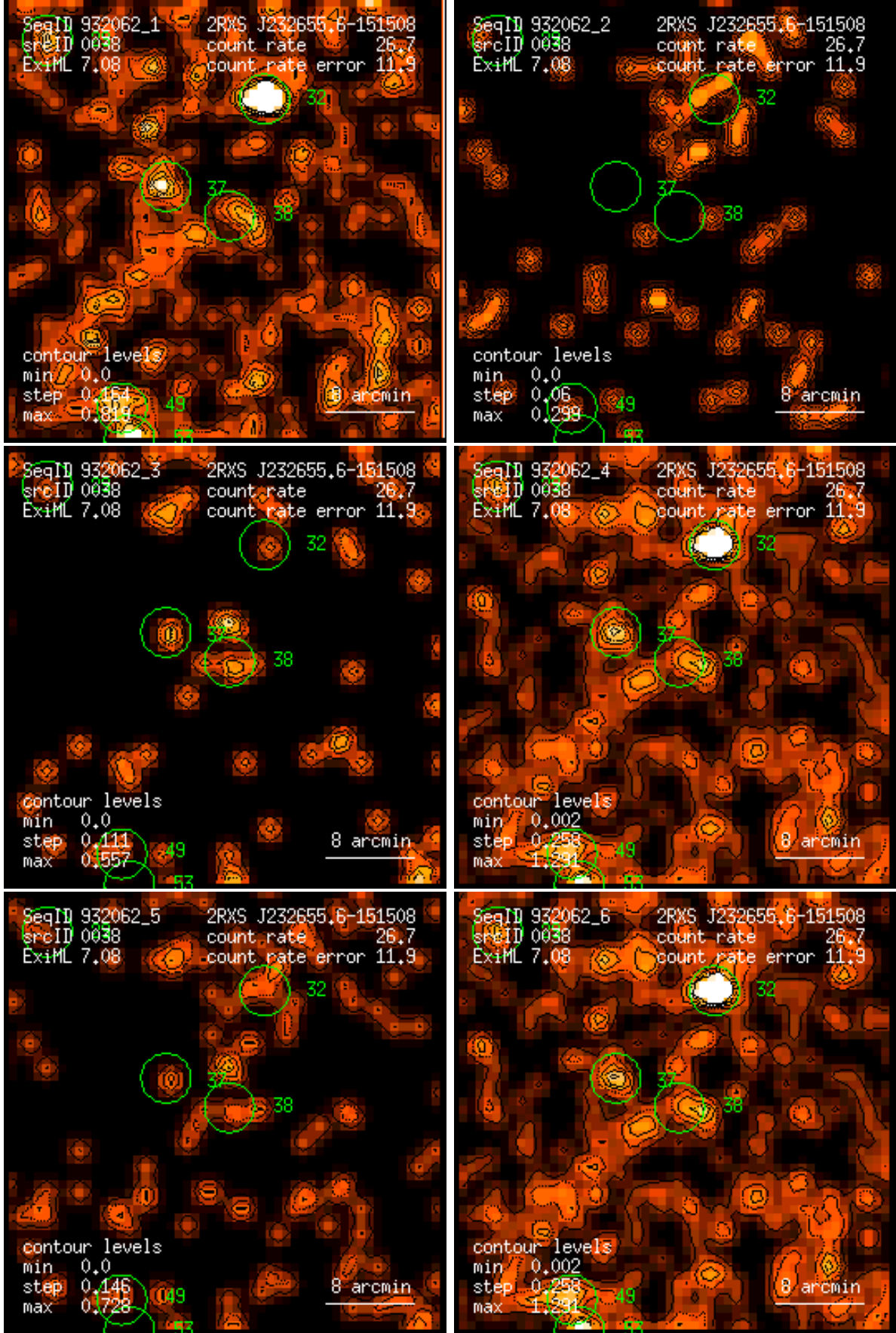
Figure 38: RASS 932062: detection 0038: band rate images, Gaussian filter: (1) PSPC channels 11 – 41, (2) 52 – 90, (3) 91 – 201, (4) 11 – 235, (5) 52 – 201, (6) 11 – 201. Broad band rates in counts/ks. Band rate contour levels in counts/ks/arcmin 2 .
