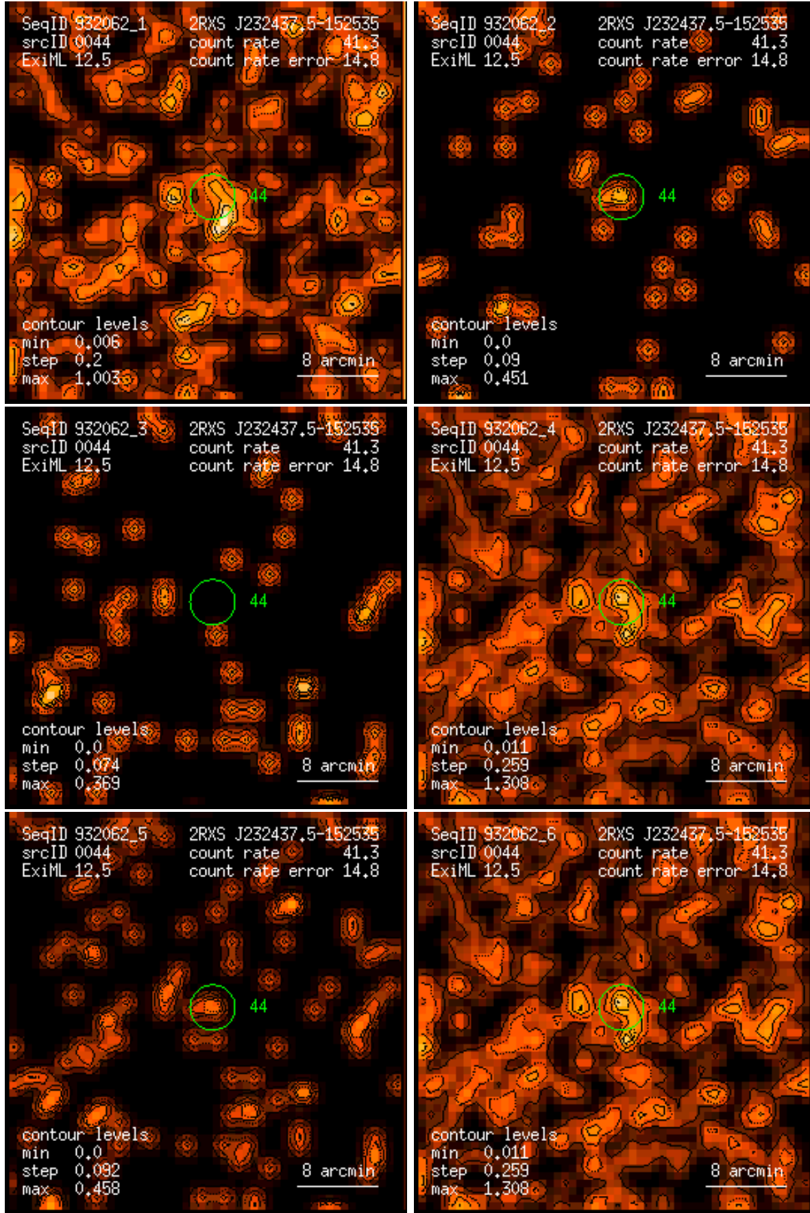
Figure 44: RASS 932062: detection 0044: band rate images, Gaussian filter: (1) PSPC channels 11 – 41, (2) 52 – 90, (3) 91 – 201, (4) 11 – 235, (5) 52 – 201, (6) 11 – 201. Broad band rates in counts/ks. Band rate contour levels in counts/ks/arcmin 2 .
