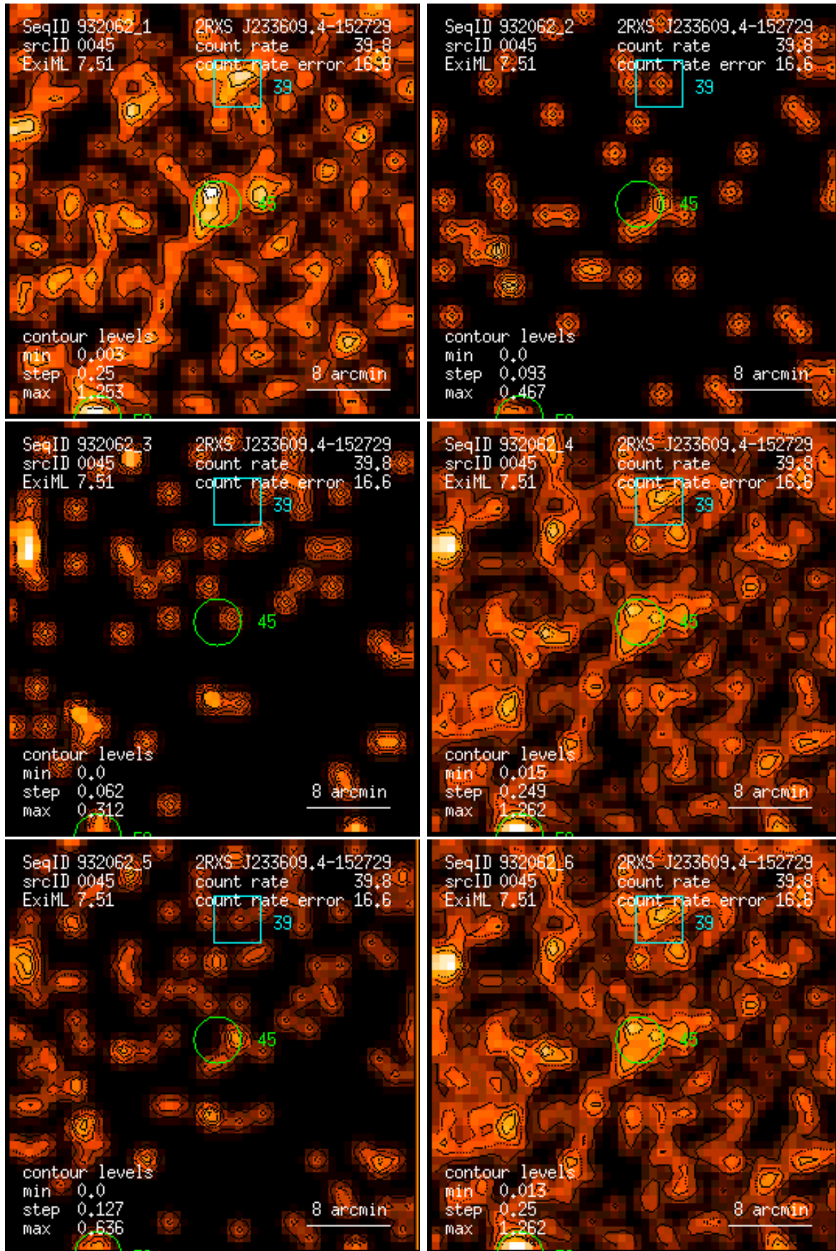
Figure 45: RASS 932062: detection 0045: band rate images, Gaussian filter: (1) PSPC channels 11 – 41, (2) 52 – 90, (3) 91 – 201, (4) 11 – 235, (5) 52 – 201, (6) 11 – 201. Broad band rates in counts/ks. Band rate contour levels in counts/ks/arcmin 2 .
