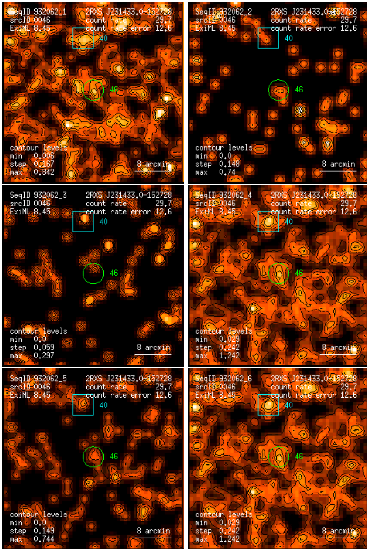
Figure 46: RASS 932062: detection 0046: band rate images, Gaussian filter: (1) PSPC channels 11 – 41, (2) 52 – 90, (3) 91 – 201, (4) 11 – 235, (5) 52 – 201, (6) 11 – 201. Broad band rates in counts/ks. Band rate contour levels in counts/ks/arcmin 2 .
