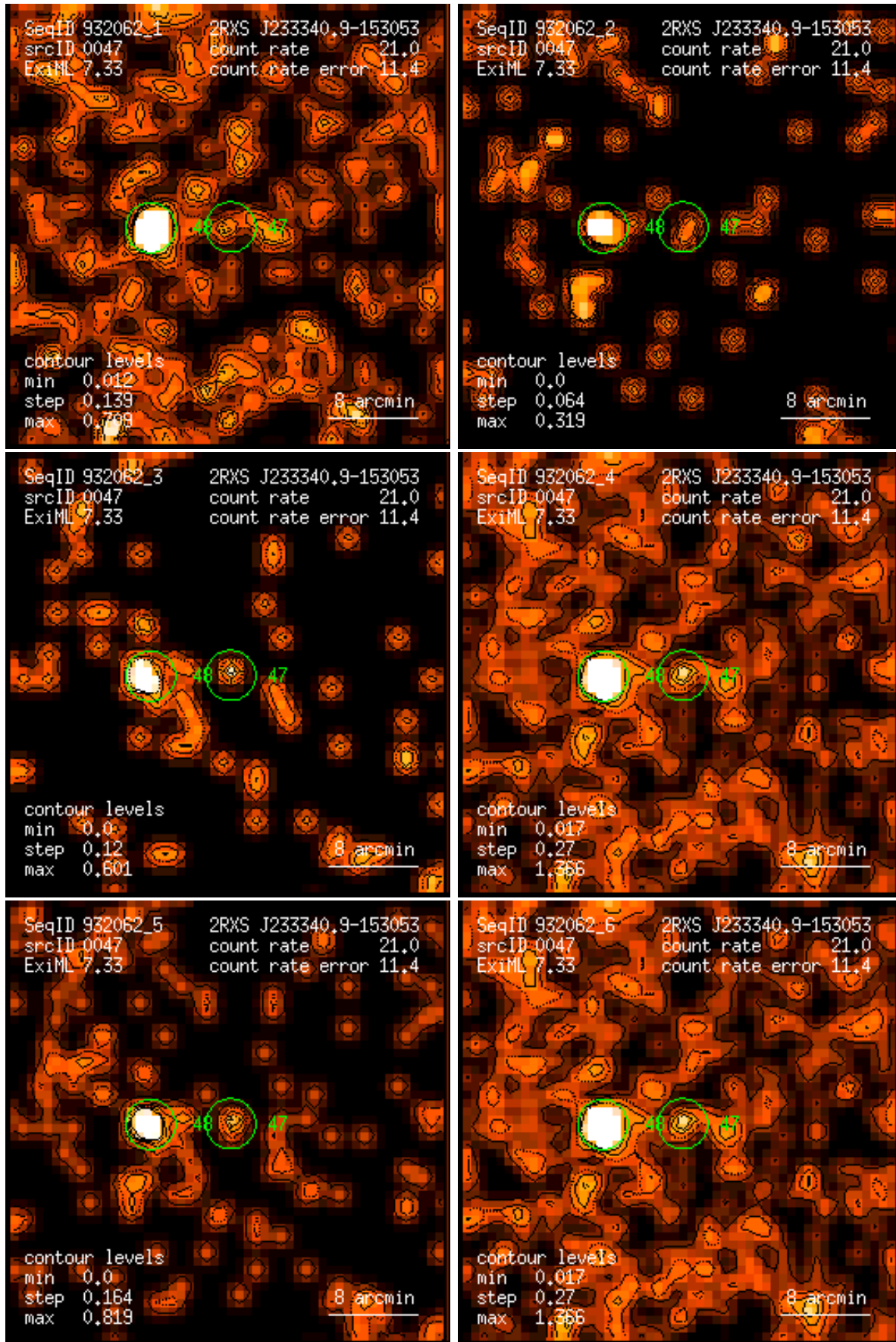
Figure 47: RASS 932062: detection 0047: band rate images, Gaussian filter: (1) PSPC channels 11 – 41, (2) 52 – 90, (3) 91 – 201, (4) 11 – 235, (5) 52 – 201, (6) 11 – 201. Broad band rates in counts/ks. Band rate contour levels in counts/ks/arcmin 2 .
