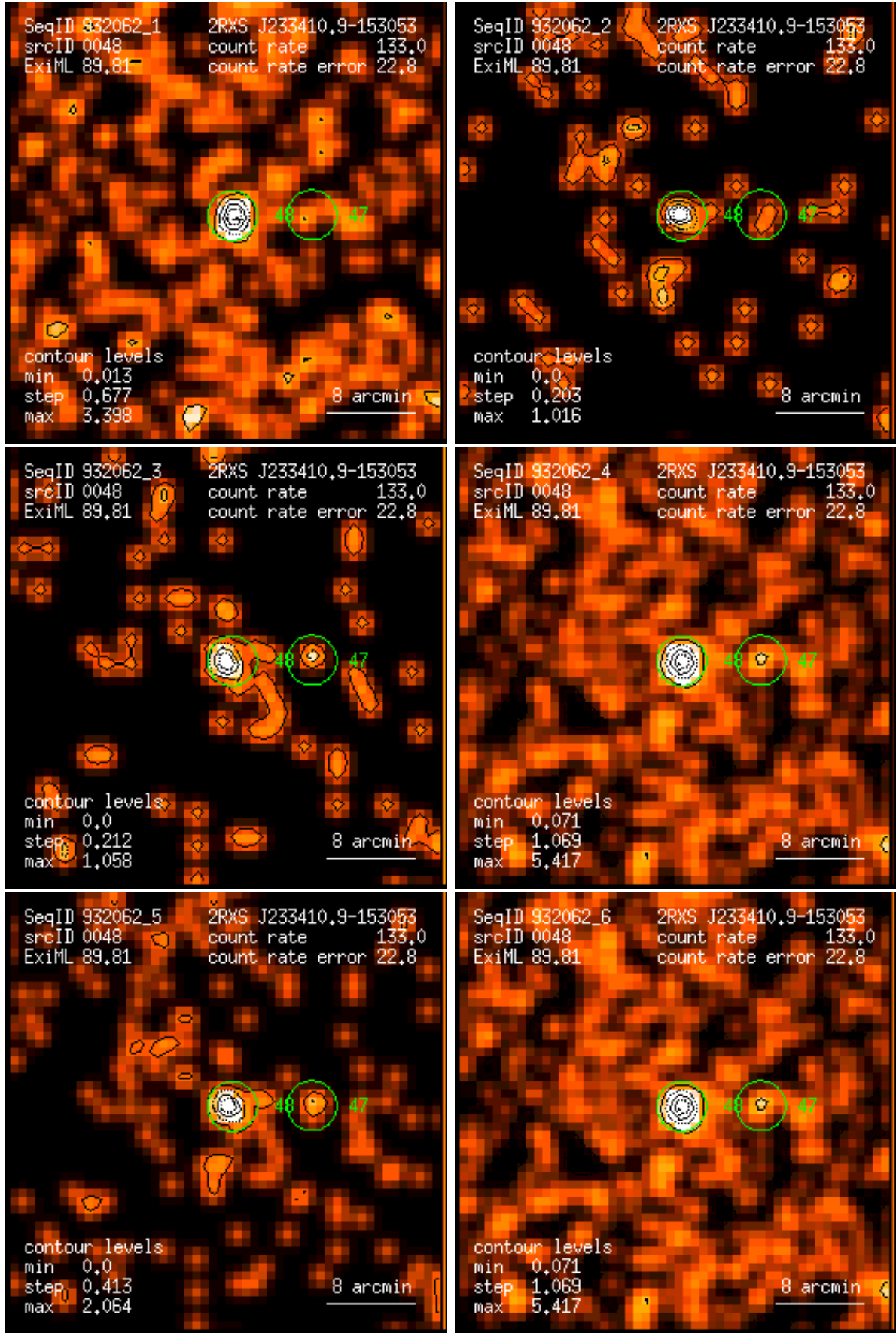
Figure 48: RASS 932062: detection 0048: band rate images, Gaussian filter: (1) PSPC channels 11 – 41, (2) 52 – 90, (3) 91 – 201, (4) 11 – 235, (5) 52 – 201, (6) 11 – 201. Broad band rates in counts/ks. Band rate contour levels in counts/ks/arcmin 2 .
