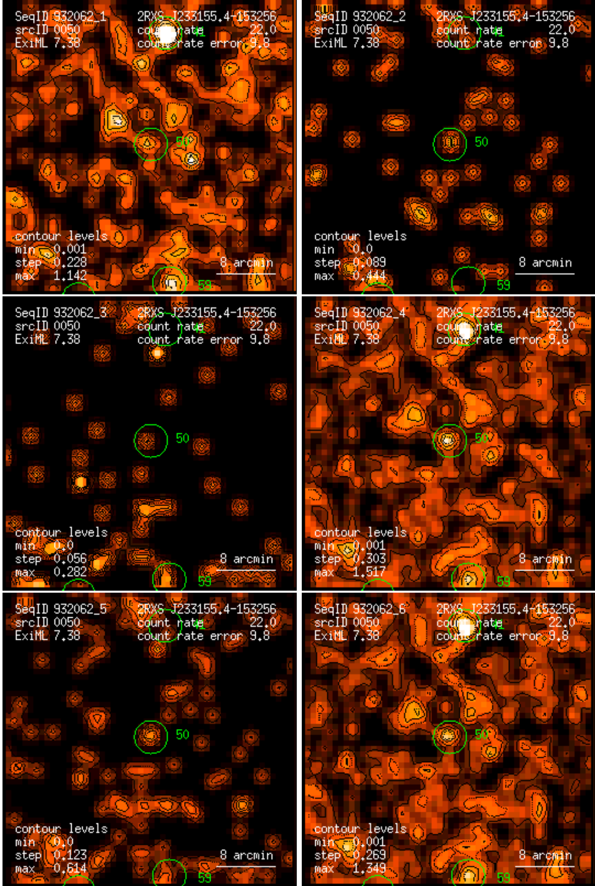
Figure 50: RASS 932062: detection 0050: band rate images, Gaussian filter: (1) PSPC channels 11 – 41, (2) 52 – 90, (3) 91 – 201, (4) 11 – 235, (5) 52 – 201, (6) 11 – 201. Broad band rates in counts/ks. Band rate contour levels in counts/ks/arcmin 2 .
