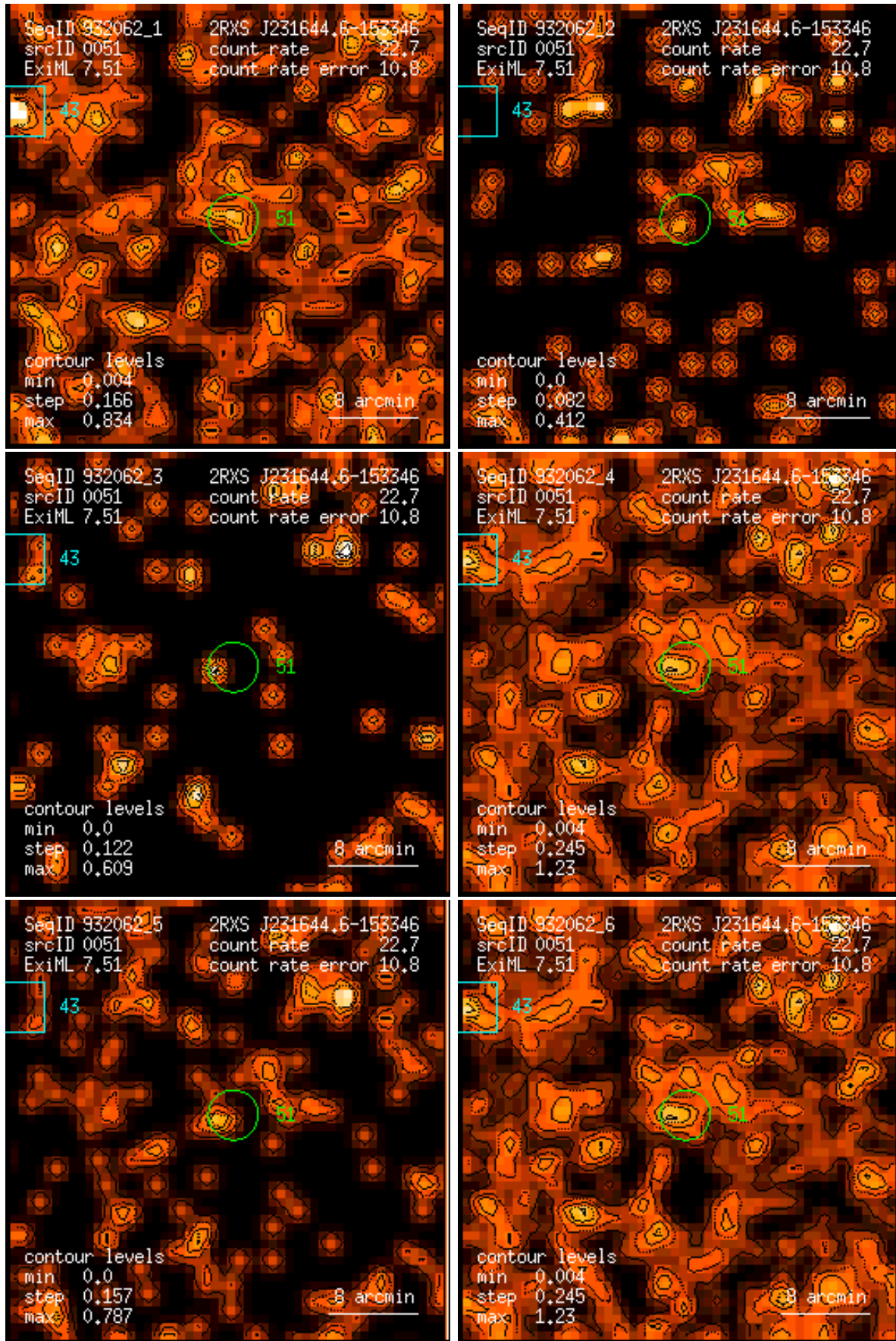
Figure 51: RASS 932062: detection 0051: band rate images, Gaussian filter: (1) PSPC channels 11 – 41, (2) 52 – 90, (3) 91 – 201, (4) 11 – 235, (5) 52 – 201, (6) 11 – 201. Broad band rates in counts/ks. Band rate contour levels in counts/ks/arcmin 2 .
