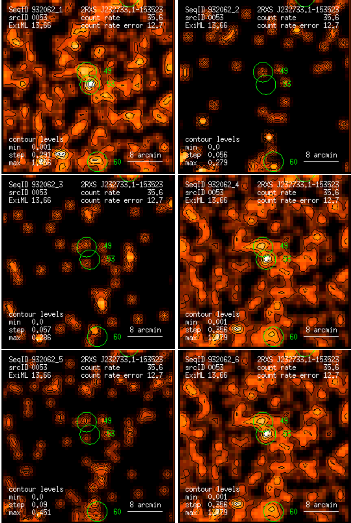
Figure 53: RASS 932062: detection 0053: band rate images, Gaussian filter: (1) PSPC channels 11 – 41, (2) 52 – 90, (3) 91 – 201, (4) 11 – 235, (5) 52 – 201, (6) 11 – 201. Broad band rates in counts/ks. Band rate contour levels in counts/ks/arcmin 2 .
