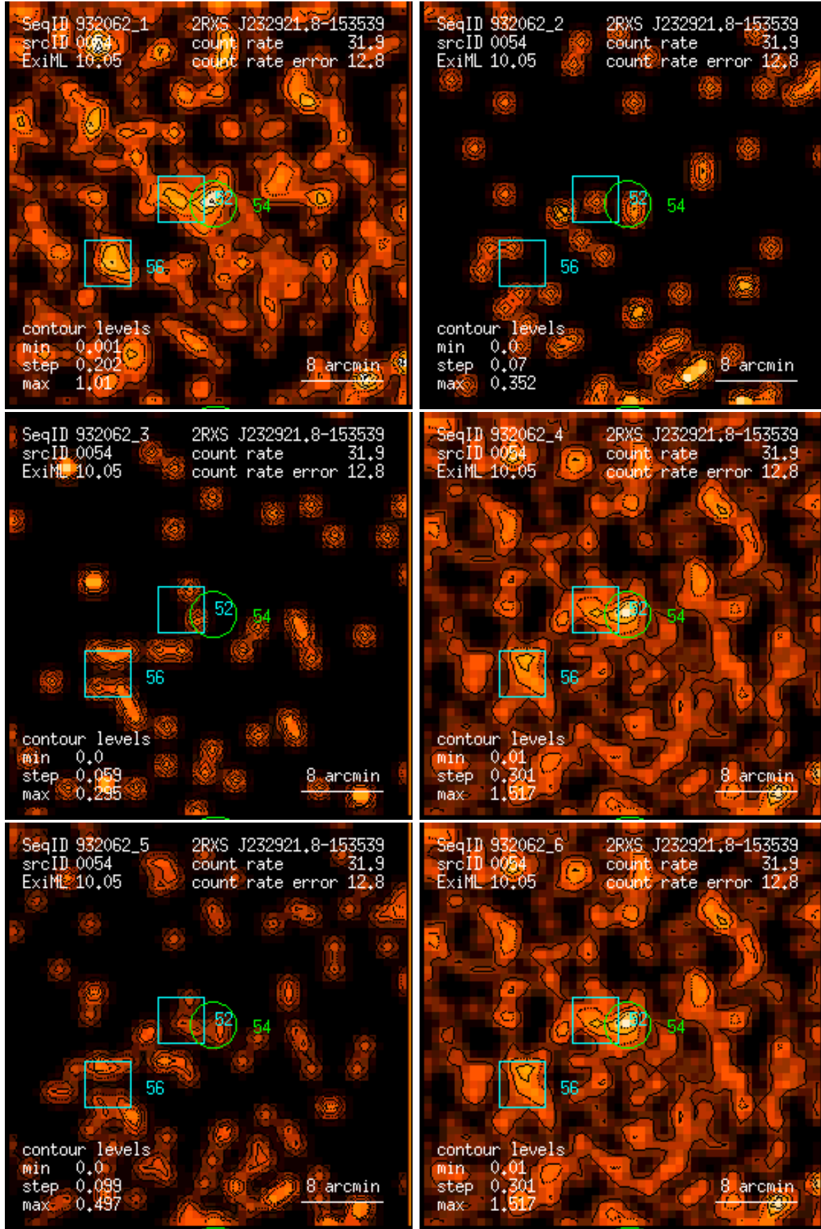
Figure 54: RASS 932062: detection 0054: band rate images, Gaussian filter: (1) PSPC channels 11 – 41, (2) 52 – 90, (3) 91 – 201, (4) 11 – 235, (5) 52 – 201, (6) 11 – 201. Broad band rates in counts/ks. Band rate contour levels in counts/ks/arcmin 2 .
