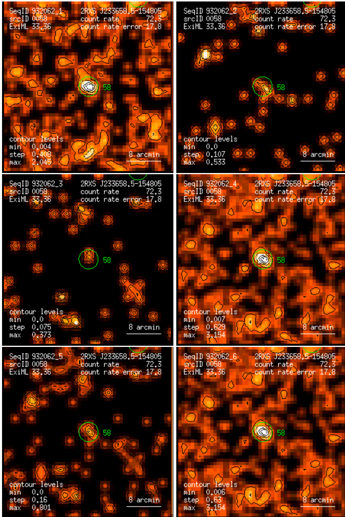
Figure 58: RASS 932062: detection 0058: band rate images, Gaussian filter: (1) PSPC channels 11 – 41, (2) 52 – 90, (3) 91 – 201, (4) 11 – 235, (5) 52 – 201, (6) 11 – 201. Broad band rates in counts/ks. Band rate contour levels in counts/ks/arcmin 2 .
