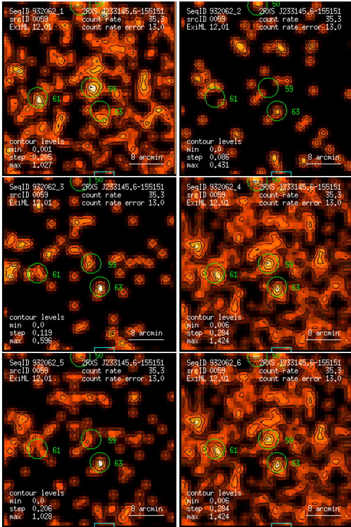
Figure 59: RASS 932062: detection 0059: band rate images, Gaussian filter: (1) PSPC channels 11 – 41, (2) 52 – 90, (3) 91 – 201, (4) 11 – 235, (5) 52 – 201, (6) 11 – 201. Broad band rates in counts/ks. Band rate contour levels in counts/ks/arcmin 2 .
