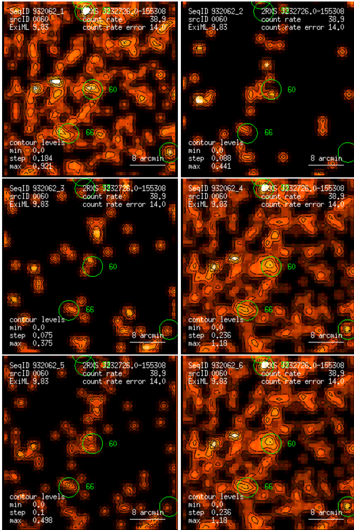
Figure 60: RASS 932062: detection 0060: band rate images, Gaussian filter: (1) PSPC channels 11 – 41, (2) 52 – 90, (3) 91 – 201, (4) 11 – 235, (5) 52 – 201, (6) 11 – 201. Broad band rates in counts/ks. Band rate contour levels in counts/ks/arcmin 2 .
