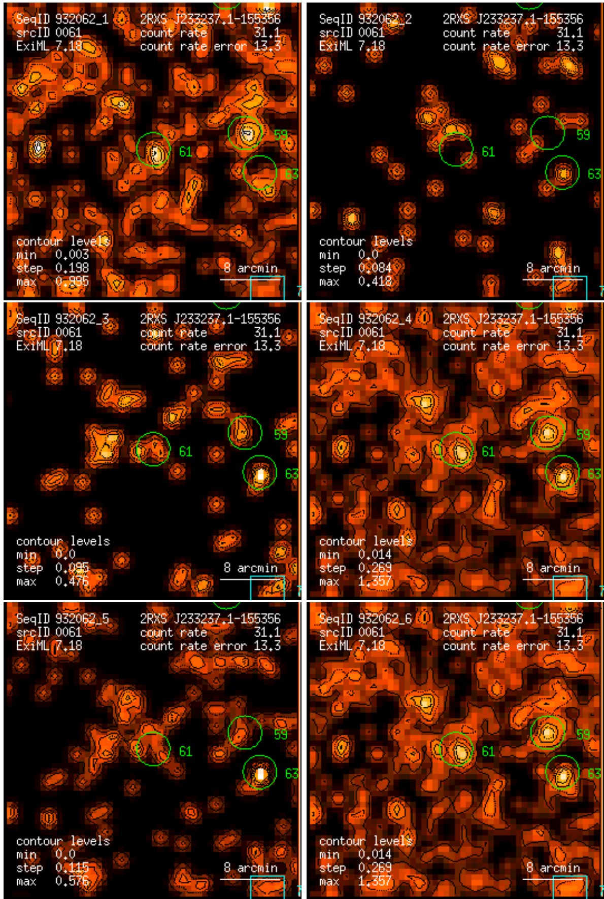
Figure 61: RASS 932062: detection 0061: band rate images, Gaussian filter: (1) PSPC channels 11 – 41, (2) 52 – 90, (3) 91 – 201, (4) 11 – 235, (5) 52 – 201, (6) 11 – 201. Broad band rates in counts/ks. Band rate contour levels in counts/ks/arcmin 2 .
