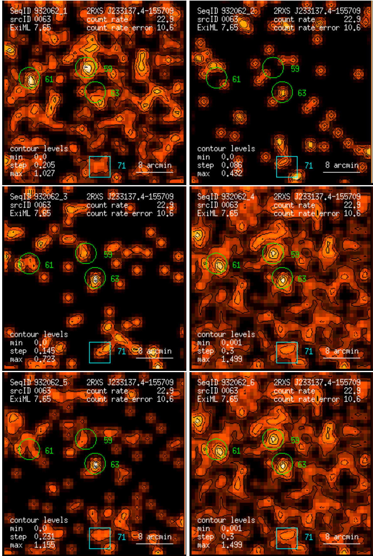
Figure 63: RASS 932062: detection 0063: band rate images, Gaussian filter: (1) PSPC channels 11 – 41, (2) 52 – 90, (3) 91 – 201, (4) 11 – 235, (5) 52 – 201, (6) 11 – 201. Broad band rates in counts/ks. Band rate contour levels in counts/ks/arcmin 2 .
