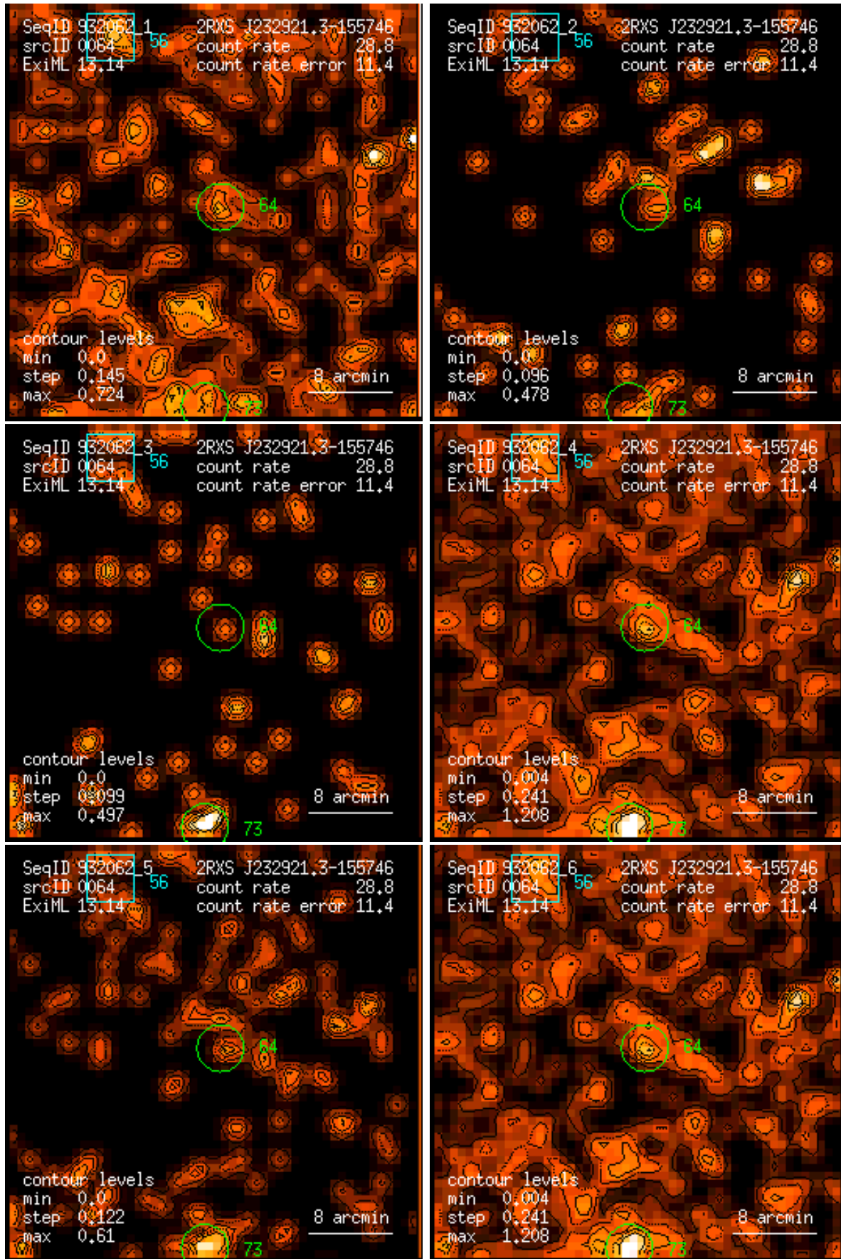
Figure 64: RASS 932062: detection 0064: band rate images, Gaussian filter: (1) PSPC channels 11 – 41, (2) 52 – 90, (3) 91 – 201, (4) 11 – 235, (5) 52 – 201, (6) 11 – 201. Broad band rates in counts/ks. Band rate contour levels in counts/ks/arcmin 2 .
