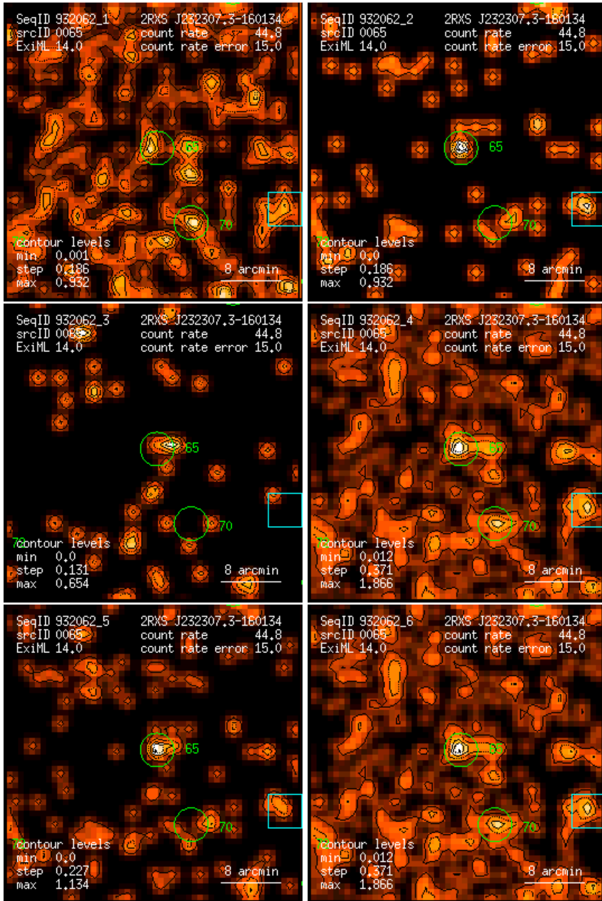
Figure 65: RASS 932062: detection 0065: band rate images, Gaussian filter: (1) PSPC channels 11 – 41, (2) 52 – 90, (3) 91 – 201, (4) 11 – 235, (5) 52 – 201, (6) 11 – 201. Broad band rates in counts/ks. Band rate contour levels in counts/ks/arcmin 2 .
