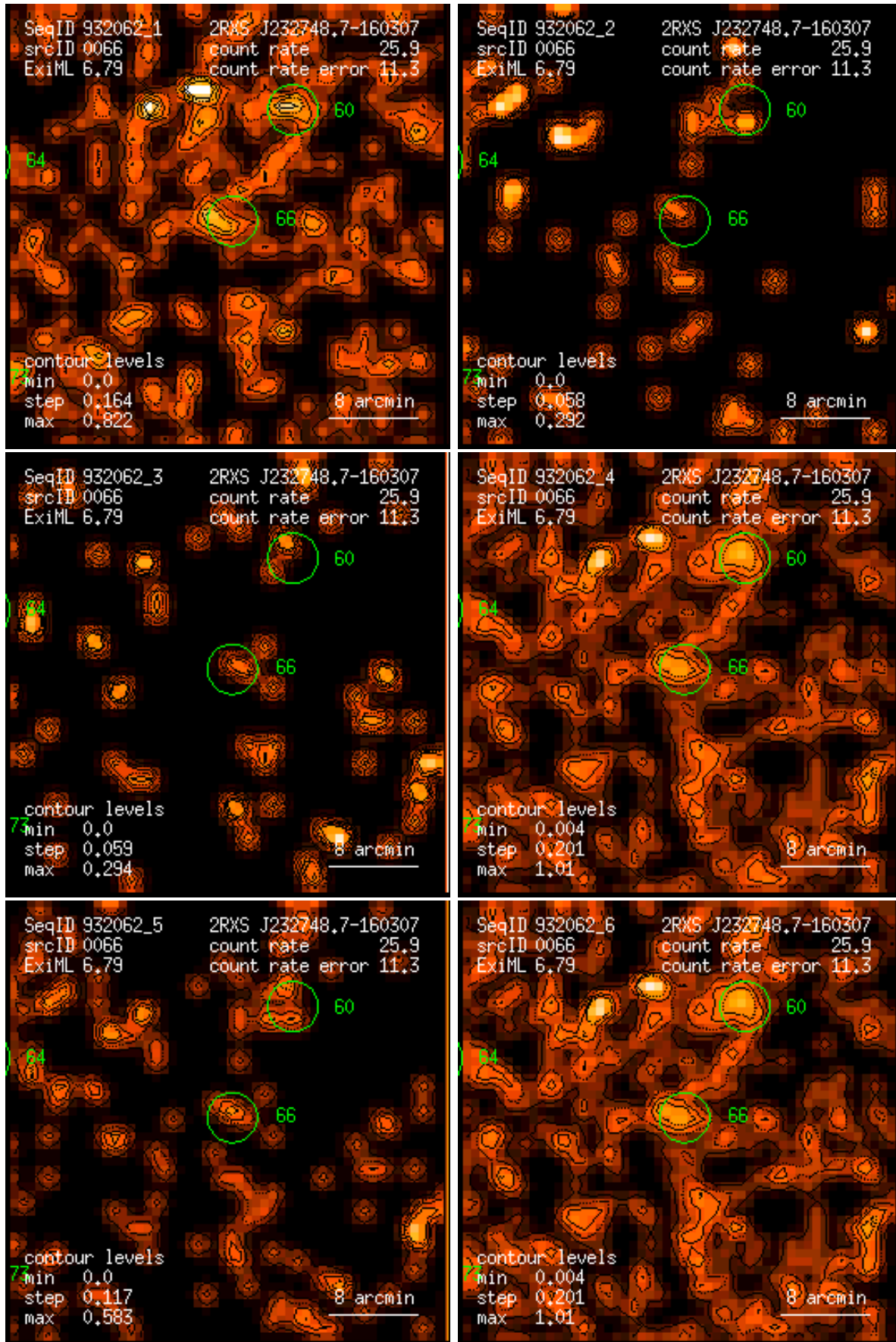
Figure 66: RASS 932062: detection 0066: band rate images, Gaussian filter: (1) PSPC channels 11 – 41, (2) 52 – 90, (3) 91 – 201, (4) 11 – 235, (5) 52 – 201, (6) 11 – 201. Broad band rates in counts/ks. Band rate contour levels in counts/ks/arcmin 2 .
