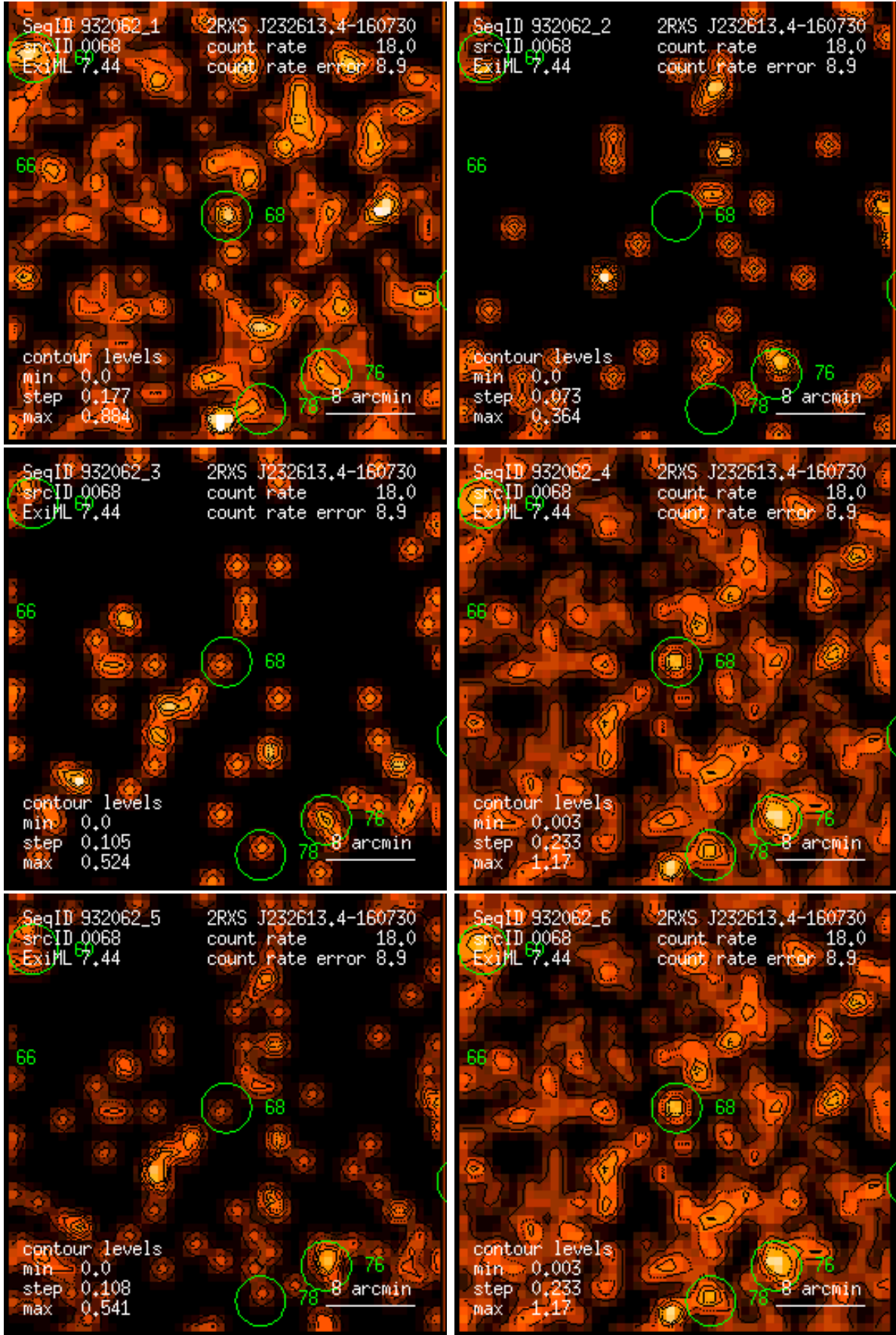
Figure 68: RASS 932062: detection 0068: band rate images, Gaussian filter: (1) PSPC channels 11 – 41, (2) 52 – 90, (3) 91 – 201, (4) 11 – 235, (5) 52 – 201, (6) 11 – 201. Broad band rates in counts/ks. Band rate contour levels in counts/ks/arcmin 2 .
