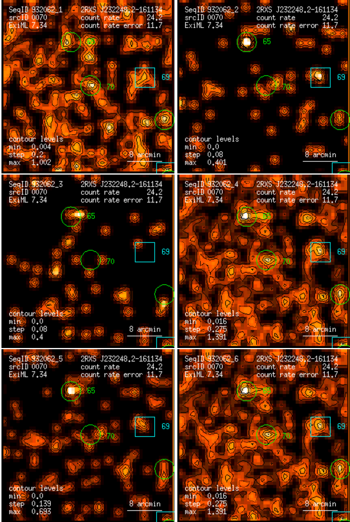
Figure 70: RASS 932062: detection 0070: band rate images, Gaussian filter: (1) PSPC channels 11 – 41, (2) 52 – 90, (3) 91 – 201, (4) 11 – 235, (5) 52 – 201, (6) 11 – 201. Broad band rates in counts/ks. Band rate contour levels in counts/ks/arcmin 2 .
