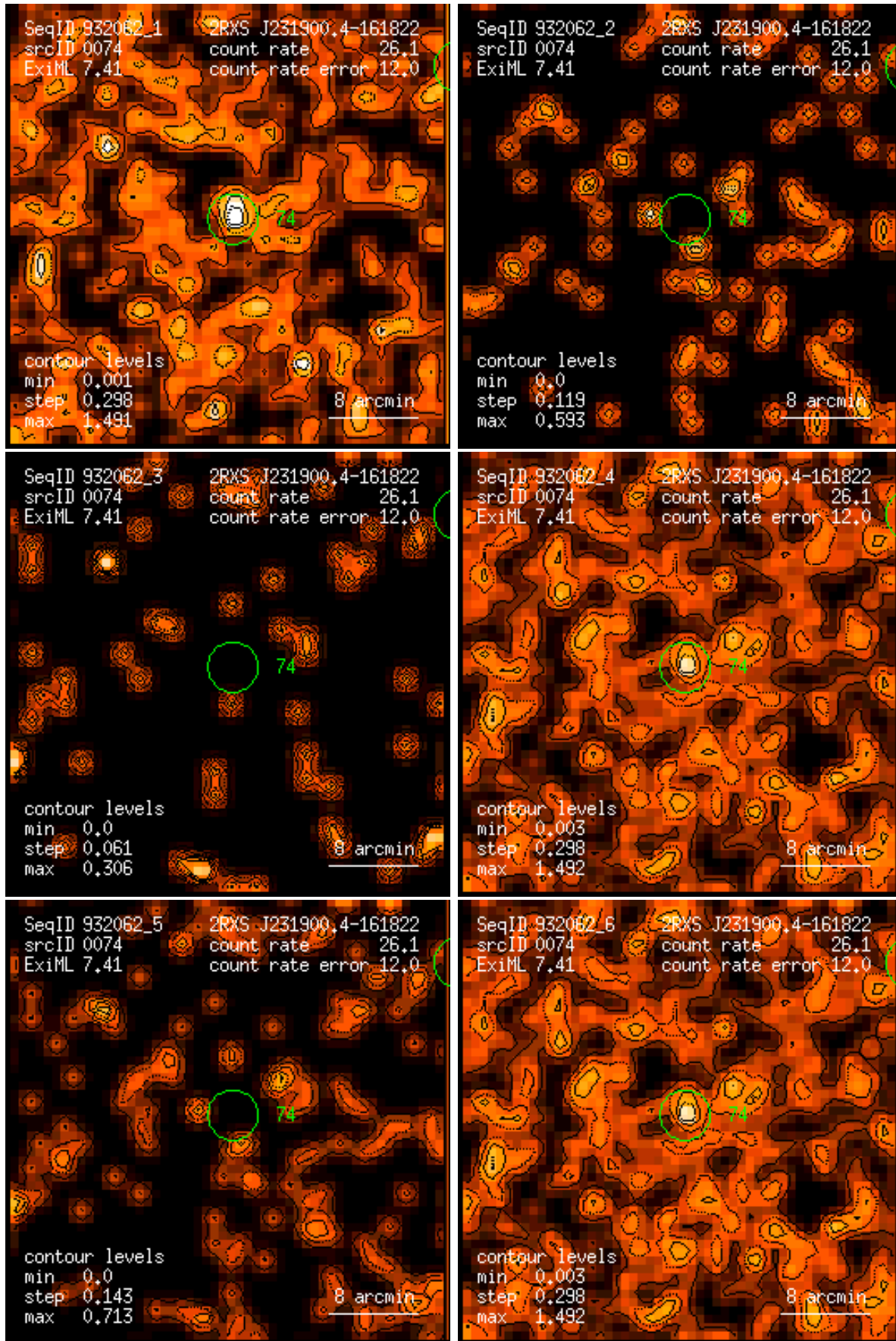
Figure 74: RASS 932062: detection 0074: band rate images, Gaussian filter: (1) PSPC channels 11 – 41, (2) 52 – 90, (3) 91 – 201, (4) 11 – 235, (5) 52 – 201, (6) 11 – 201. Broad band rates in counts/ks. Band rate contour levels in counts/ks/arcmin 2 .
