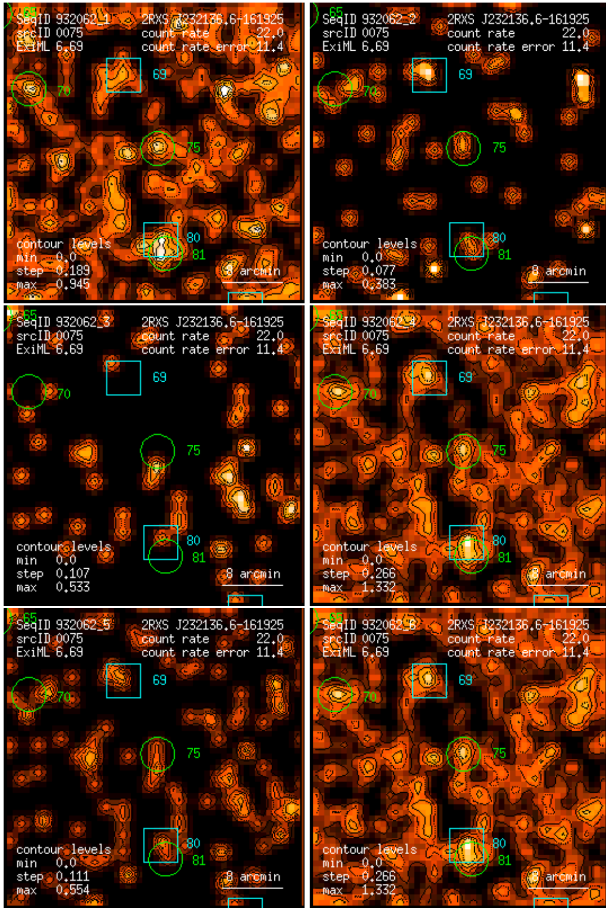
Figure 75: RASS 932062: detection 0075: band rate images, Gaussian filter: (1) PSPC channels 11 – 41, (2) 52 – 90, (3) 91 – 201, (4) 11 – 235, (5) 52 – 201, (6) 11 – 201. Broad band rates in counts/ks. Band rate contour levels in counts/ks/arcmin 2 .
