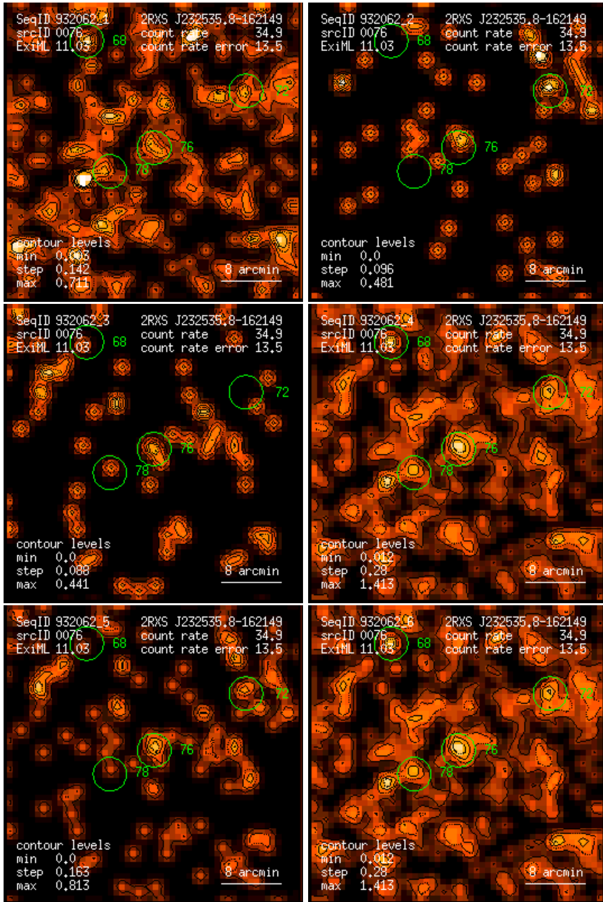
Figure 76: RASS 932062: detection 0076: band rate images, Gaussian filter: (1) PSPC channels 11 – 41, (2) 52 – 90, (3) 91 – 201, (4) 11 – 235, (5) 52 – 201, (6) 11 – 201. Broad band rates in counts/ks. Band rate contour levels in counts/ks/arcmin 2 .
