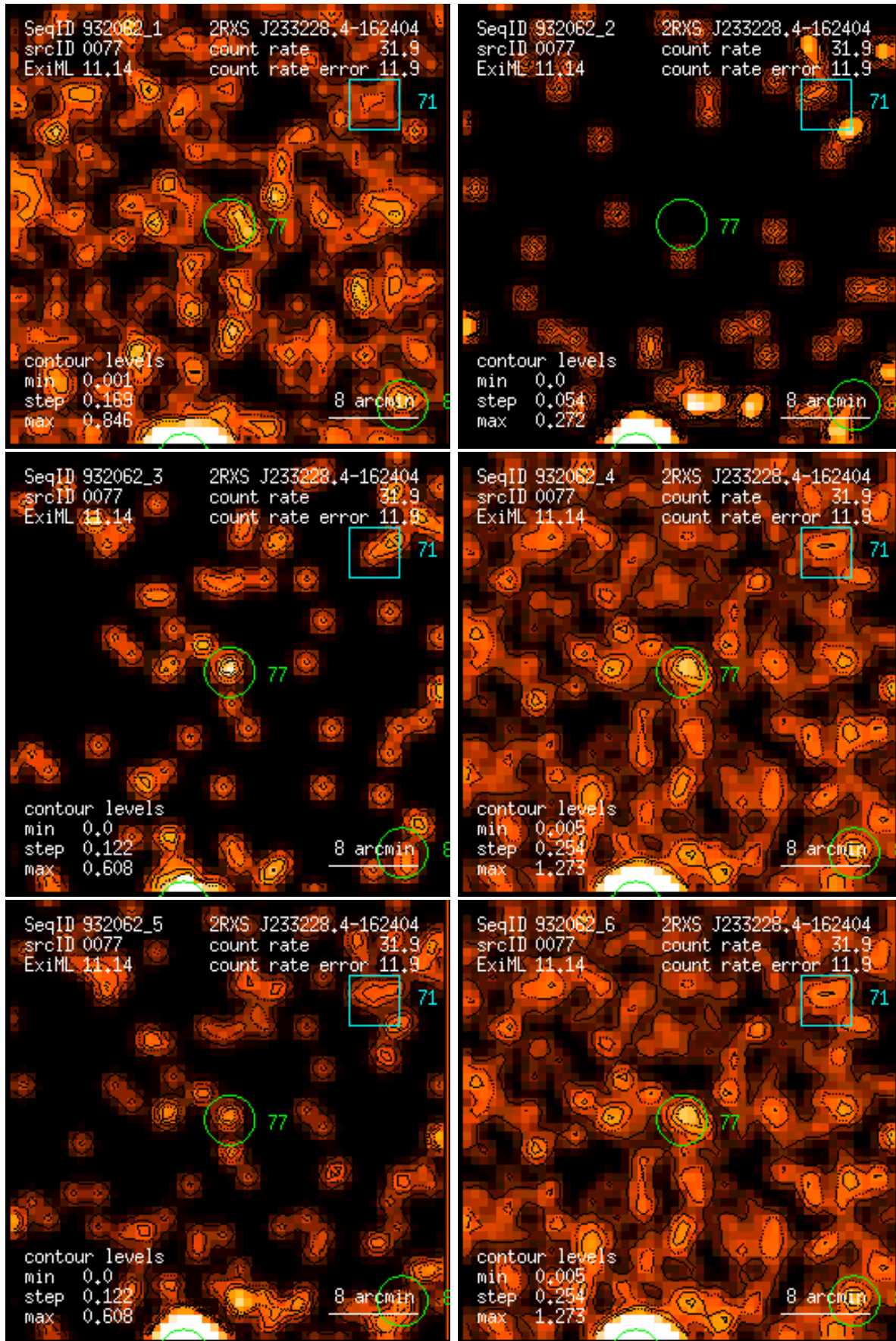
Figure 77: RASS 932062: detection 0077: band rate images, Gaussian filter: (1) PSPC channels 11 – 41, (2) 52 – 90, (3) 91 – 201, (4) 11 – 235, (5) 52 – 201, (6) 11 – 201. Broad band rates in counts/ks. Band rate contour levels in counts/ks/arcmin 2 .
