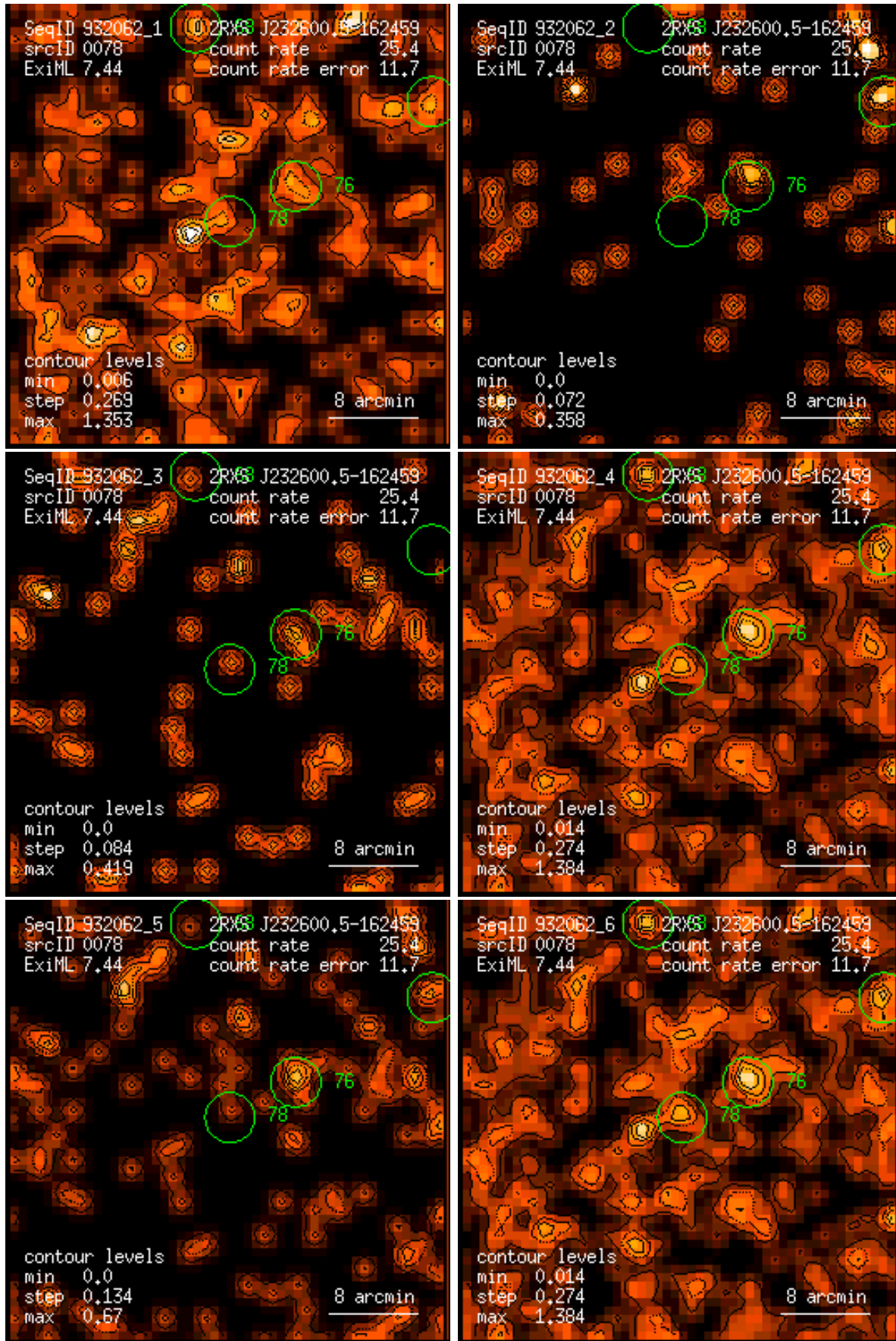
Figure 78: RASS 932062: detection 0078: band rate images, Gaussian filter: (1) PSPC channels 11 – 41, (2) 52 – 90, (3) 91 – 201, (4) 11 – 235, (5) 52 – 201, (6) 11 – 201. Broad band rates in counts/ks. Band rate contour levels in counts/ks/arcmin 2 .
