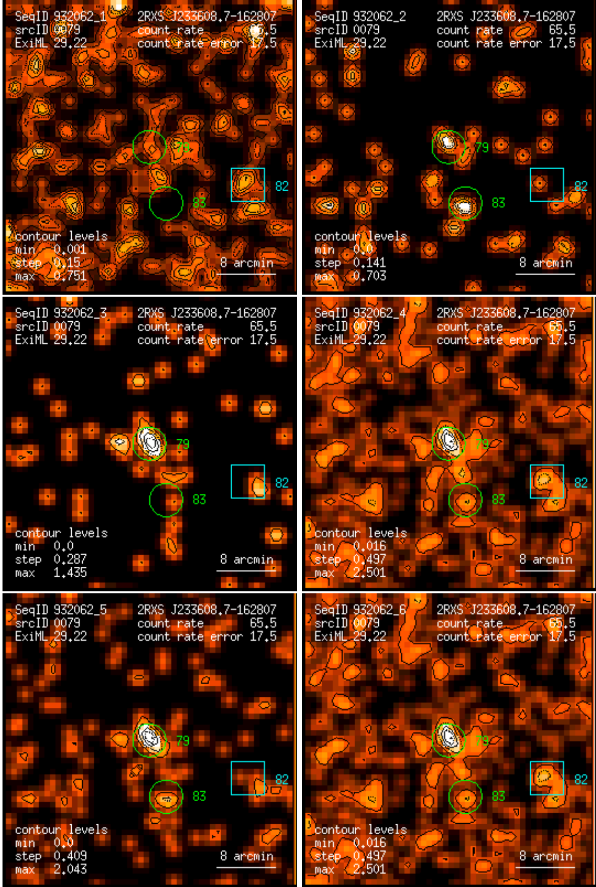
Figure 79: RASS 932062: detection 0079: band rate images, Gaussian filter: (1) PSPC channels 11 – 41, (2) 52 – 90, (3) 91 – 201, (4) 11 – 235, (5) 52 – 201, (6) 11 – 201. Broad band rates in counts/ks. Band rate contour levels in counts/ks/arcmin 2 .
