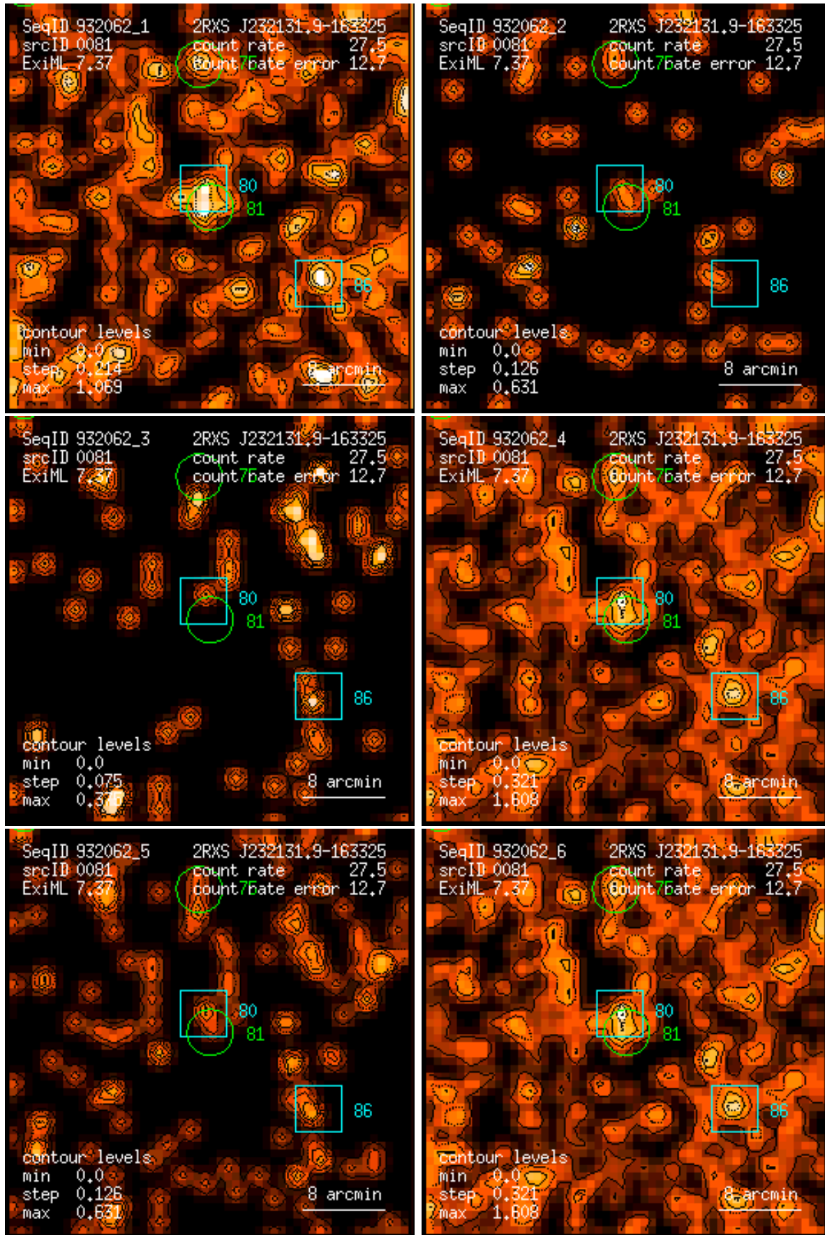
Figure 81: RASS 932062: detection 0081: band rate images, Gaussian filter: (1) PSPC channels 11 – 41, (2) 52 – 90, (3) 91 – 201, (4) 11 – 235, (5) 52 – 201, (6) 11 – 201. Broad band rates in counts/ks. Band rate contour levels in counts/ks/arcmin 2 .
