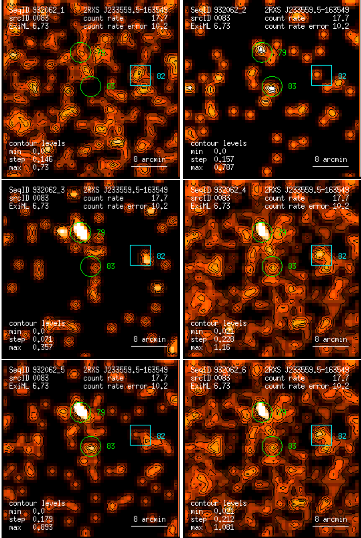
Figure 83: RASS 932062: detection 0083: band rate images, Gaussian filter: (1) PSPC channels 11 – 41, (2) 52 – 90, (3) 91 – 201, (4) 11 – 235, (5) 52 – 201, (6) 11 – 201. Broad band rates in counts/ks. Band rate contour levels in counts/ks/arcmin 2 .
