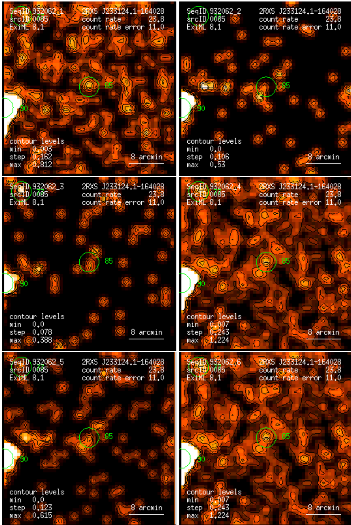
Figure 85: RASS 932062: detection 0085: band rate images, Gaussian filter: (1) PSPC channels 11 – 41, (2) 52 – 90, (3) 91 – 201, (4) 11 – 235, (5) 52 – 201, (6) 11 – 201. Broad band rates in counts/ks. Band rate contour levels in counts/ks/arcmin 2 .
