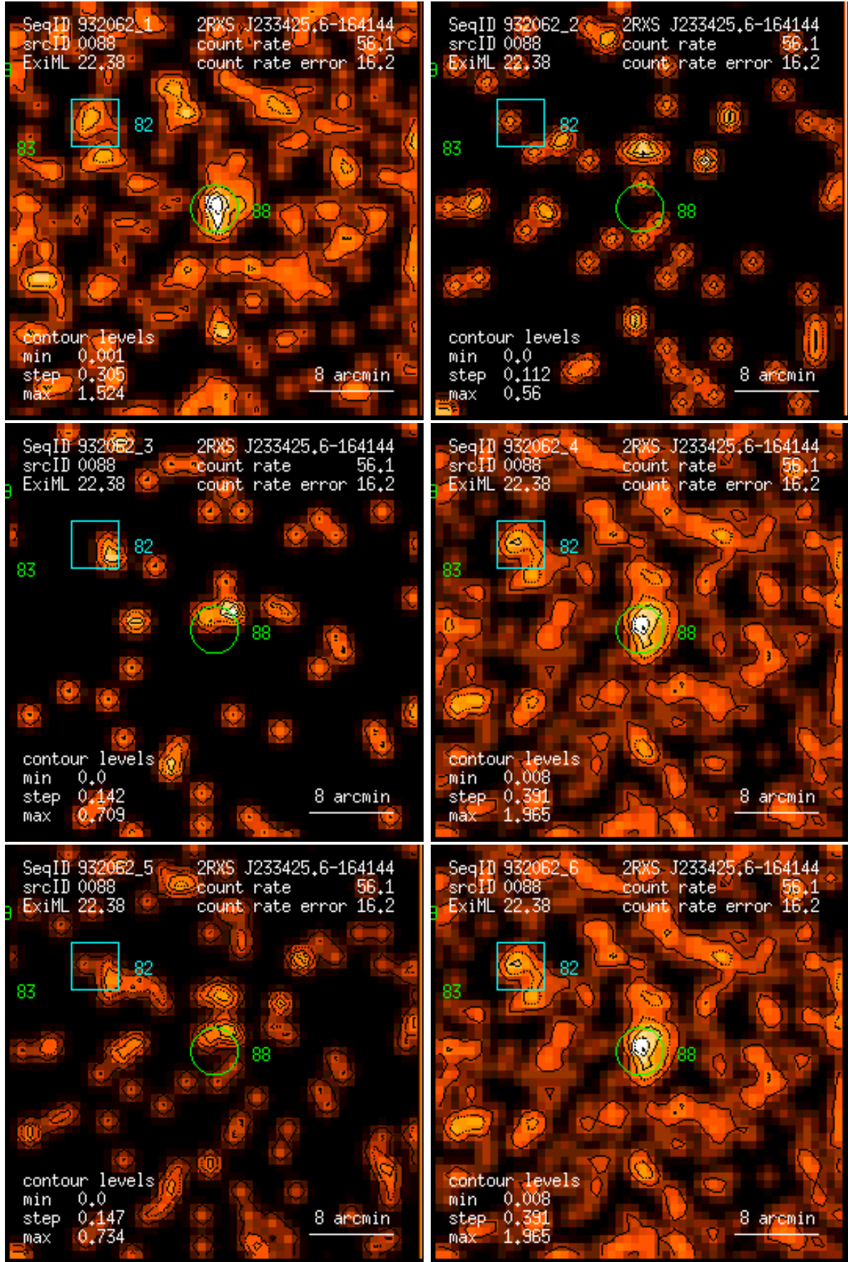
Figure 88: RASS 932062: detection 0088: band rate images, Gaussian filter: (1) PSPC channels 11 – 41, (2) 52 – 90, (3) 91 – 201, (4) 11 – 235, (5) 52 – 201, (6) 11 – 201. Broad band rates in counts/ks. Band rate contour levels in counts/ks/arcmin 2 .
