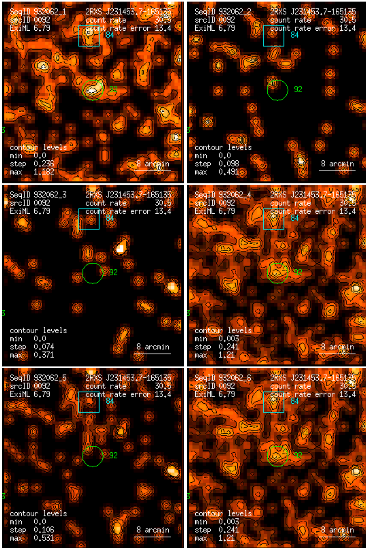
Figure 92: RASS 932062: detection 0092: band rate images, Gaussian filter: (1) PSPC channels 11 – 41, (2) 52 – 90, (3) 91 – 201, (4) 11 – 235, (5) 52 – 201, (6) 11 – 201. Broad band rates in counts/ks. Band rate contour levels in counts/ks/arcmin 2 .
