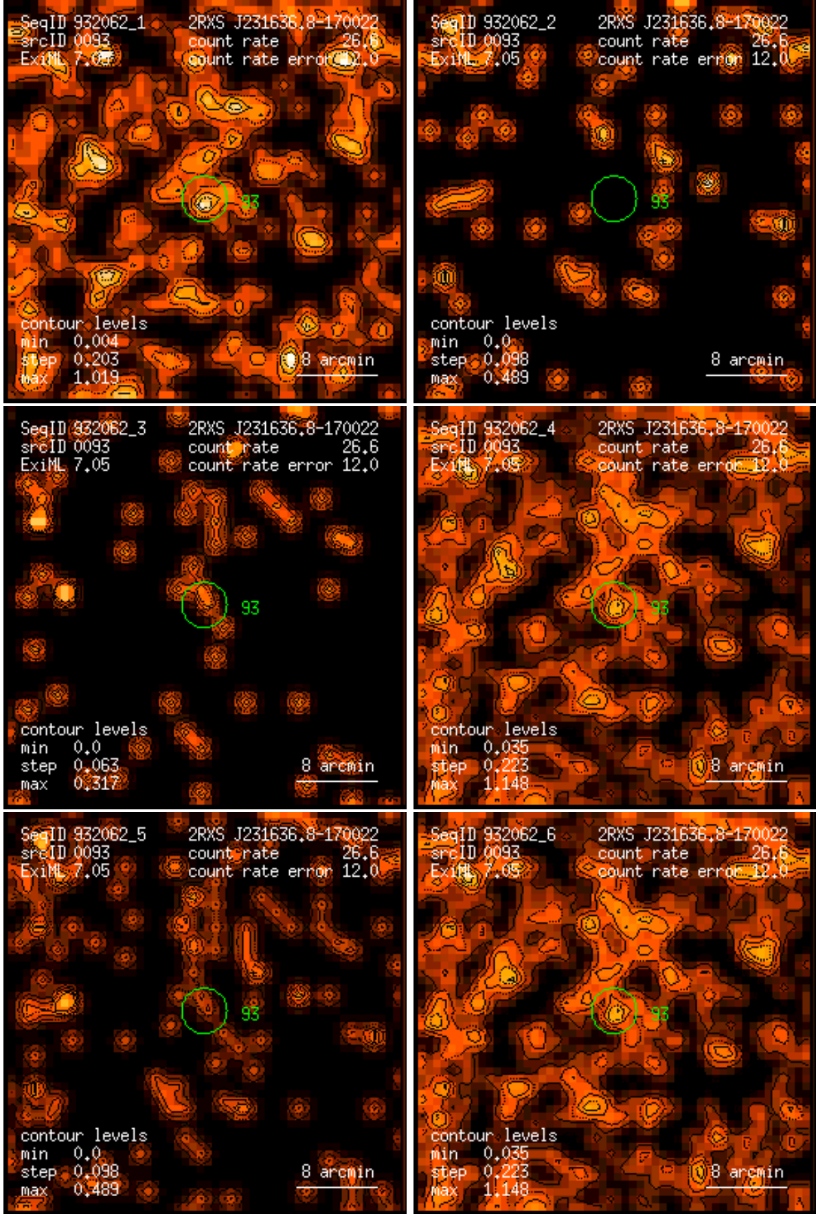
Figure 93: RASS 932062: detection 0093: band rate images, Gaussian filter: (1) PSPC channels 11 – 41, (2) 52 – 90, (3) 91 – 201, (4) 11 – 235, (5) 52 – 201, (6) 11 – 201. Broad band rates in counts/ks. Band rate contour levels in counts/ks/arcmin 2 .
