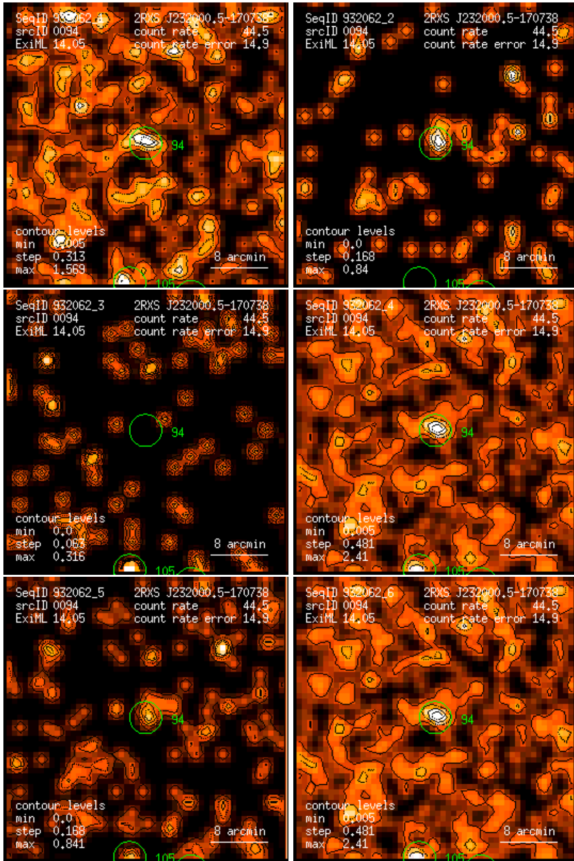
Figure 94: RASS 932062: detection 0094: band rate images, Gaussian filter: (1) PSPC channels 11 – 41, (2) 52 – 90, (3) 91 – 201, (4) 11 – 235, (5) 52 – 201, (6) 11 – 201. Broad band rates in counts/ks. Band rate contour levels in counts/ks/arcmin 2 .
