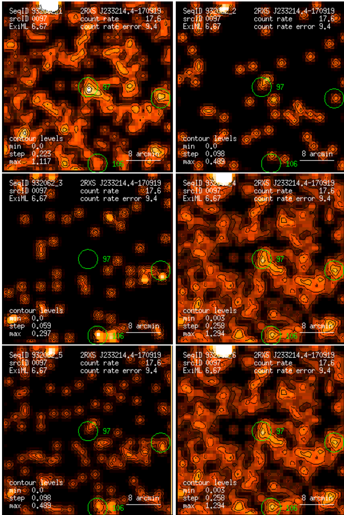
Figure 97: RASS 932062: detection 0097: band rate images, Gaussian filter: (1) PSPC channels 11 – 41, (2) 52 – 90, (3) 91 – 201, (4) 11 – 235, (5) 52 – 201, (6) 11 – 201. Broad band rates in counts/ks. Band rate contour levels in counts/ks/arcmin 2 .
