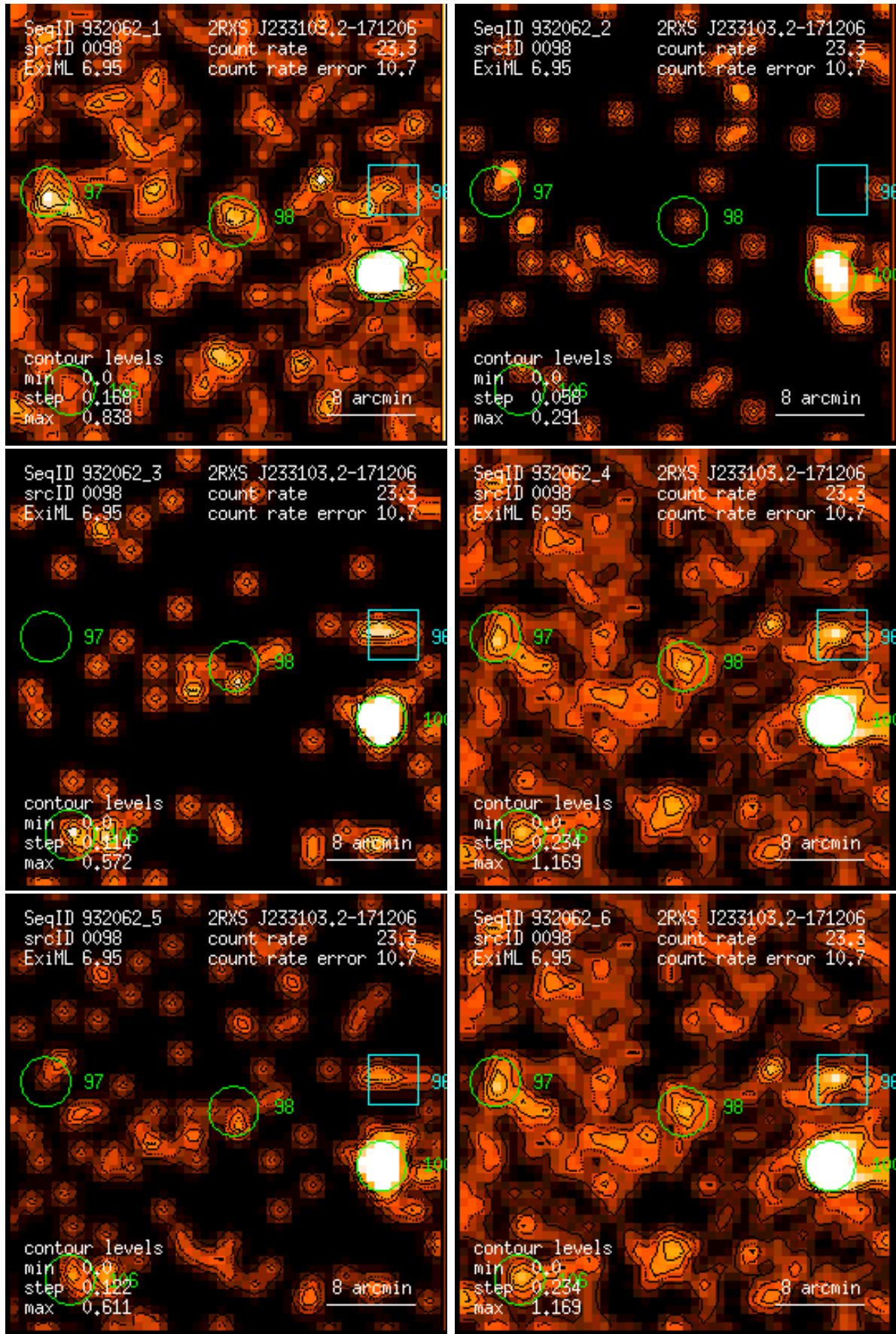
Figure 98: RASS 932062: detection 0098: band rate images, Gaussian filter: (1) PSPC channels 11 – 41, (2) 52 – 90, (3) 91 – 201, (4) 11 – 235, (5) 52 – 201, (6) 11 – 201. Broad band rates in counts/ks. Band rate contour levels in counts/ks/arcmin 2 .
