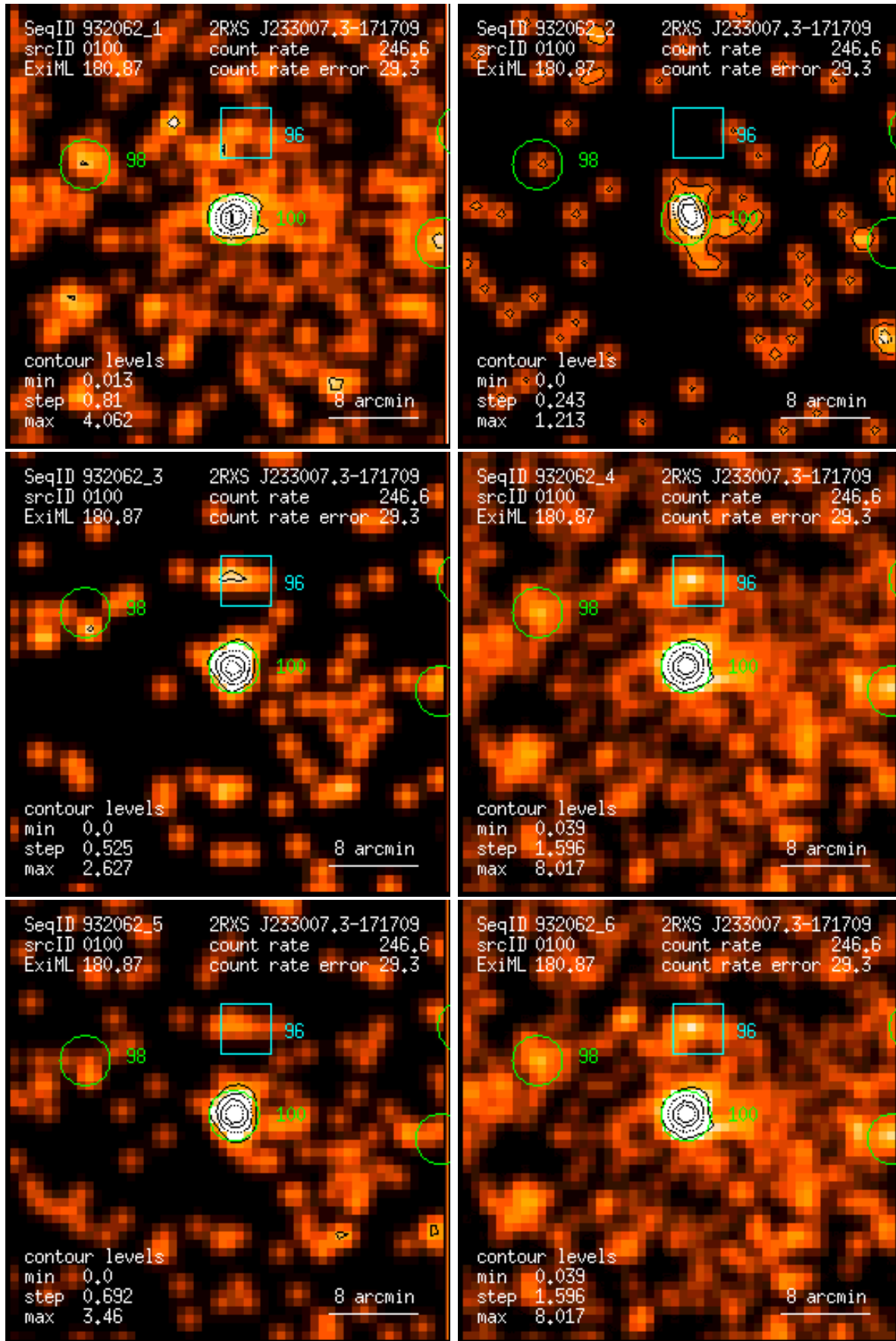
Figure 100: RASS 932062: detection 0100: band rate images, Gaussian filter: (1) PSPC channels 11 – 41, (2) 52 – 90, (3) 91 – 201, (4) 11 – 235, (5) 52 – 201, (6) 11 – 201. Broad band rates in counts/ks. Band rate contour levels in counts/ks/arcmin 2 .
