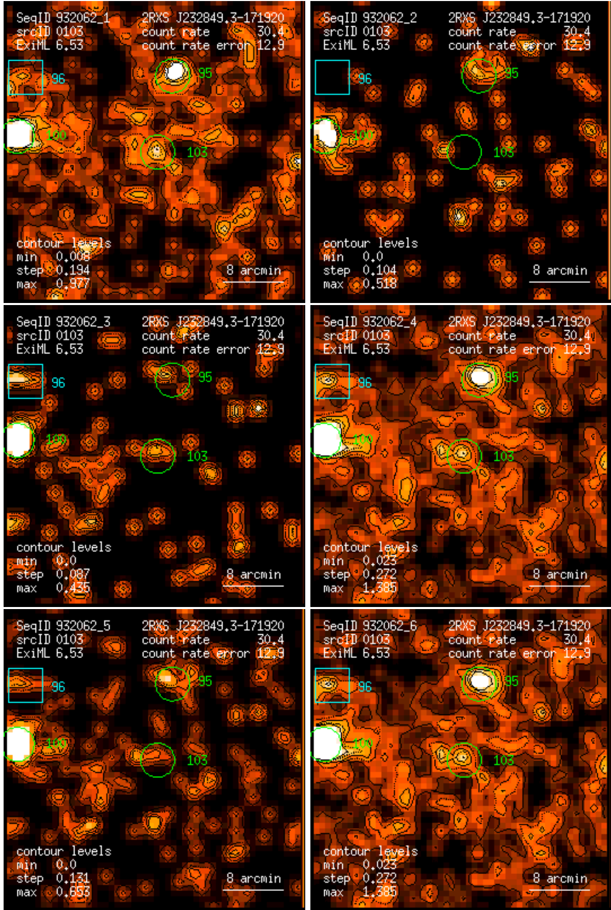
Figure 103: RASS 932062: detection 0103: band rate images, Gaussian filter: (1) PSPC channels 11 – 41, (2) 52 – 90, (3) 91 – 201, (4) 11 – 235, (5) 52 – 201, (6) 11 – 201. Broad band rates in counts/ks. Band rate contour levels in counts/ks/arcmin 2 .
