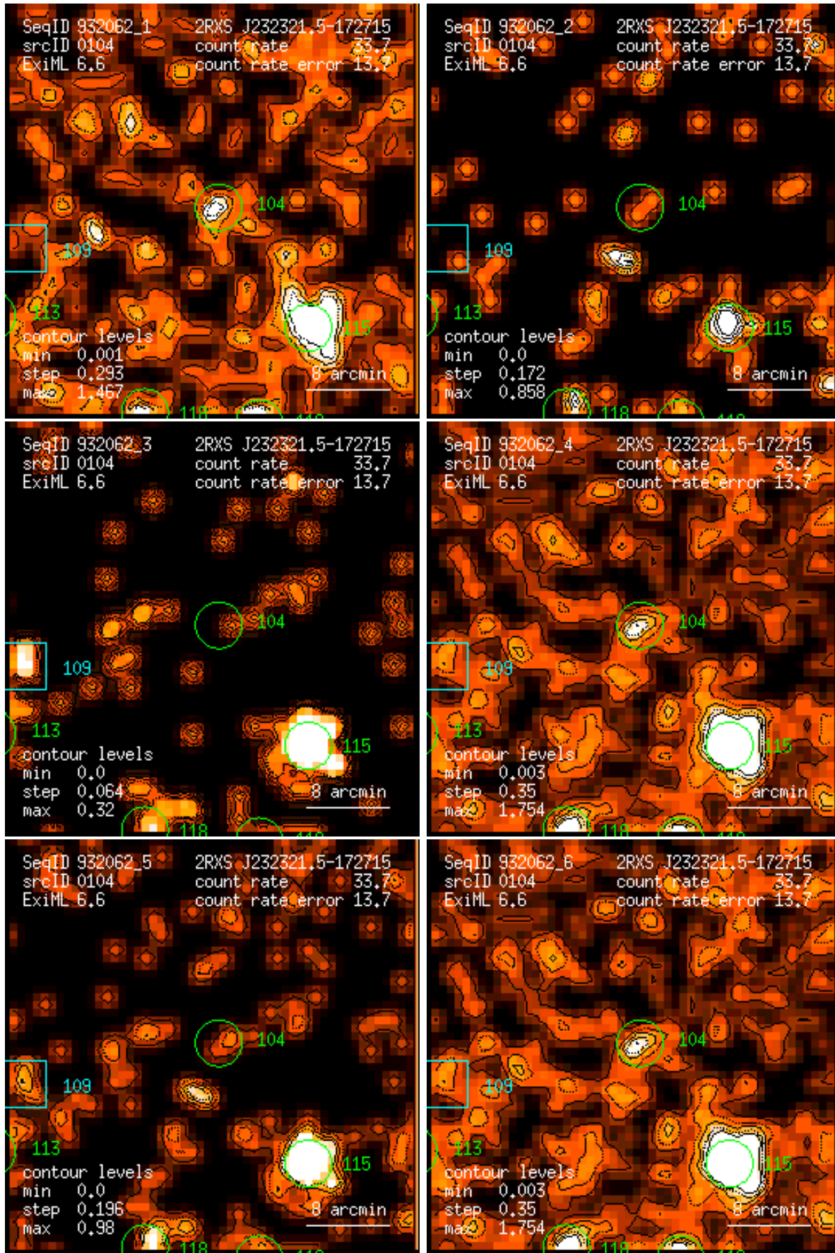
Figure 104: RASS 932062: detection 0104: band rate images, Gaussian filter: (1) PSPC channels 11 – 41, (2) 52 – 90, (3) 91 – 201, (4) 11 – 235, (5) 52 – 201, (6) 11 – 201. Broad band rates in counts/ks. Band rate contour levels in counts/ks/arcmin 2 .
