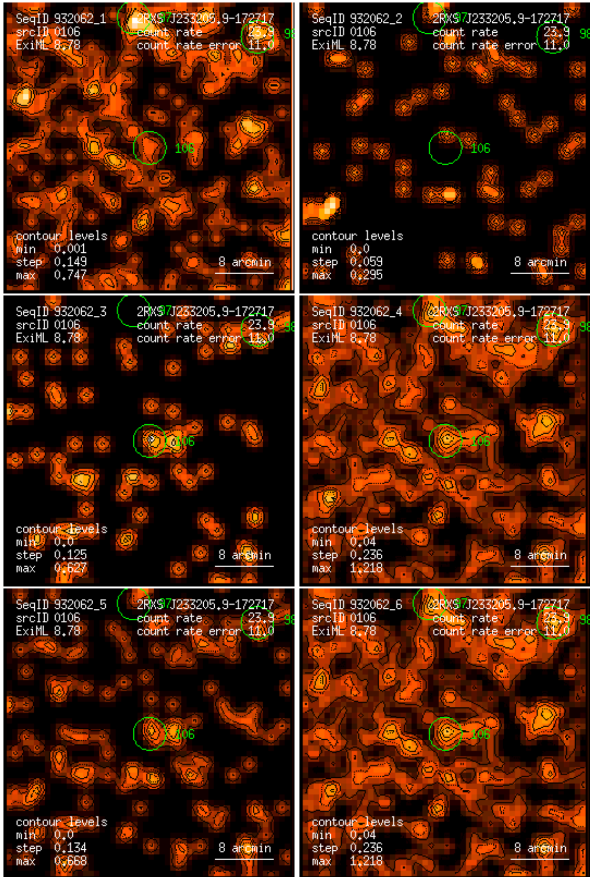
Figure 106: RASS 932062: detection 0106: band rate images, Gaussian filter: (1) PSPC channels 11 – 41, (2) 52 – 90, (3) 91 – 201, (4) 11 – 235, (5) 52 – 201, (6) 11 – 201. Broad band rates in counts/ks. Band rate contour levels in counts/ks/arcmin 2 .
