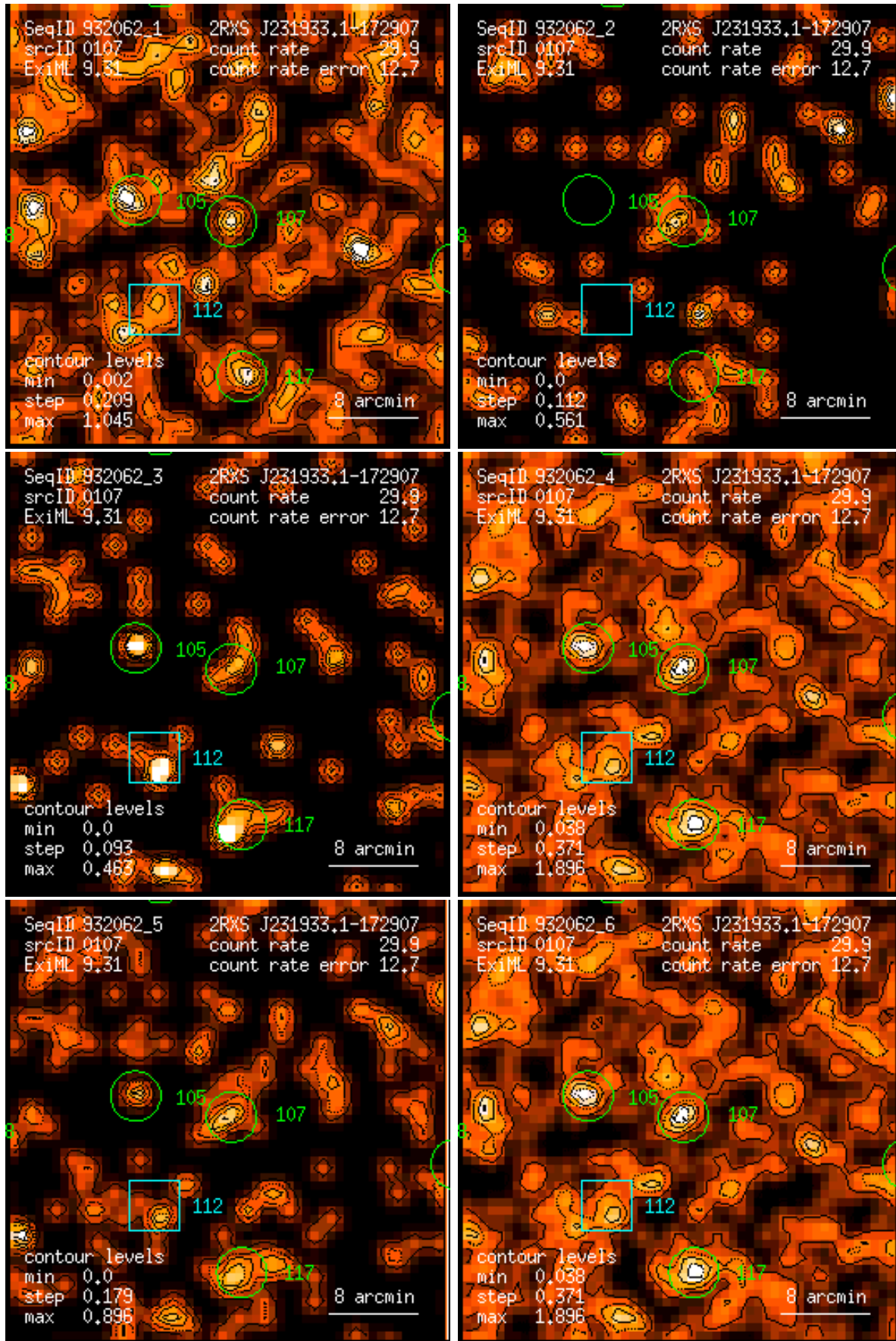
Figure 107: RASS 932062: detection 0107: band rate images, Gaussian filter: (1) PSPC channels 11 – 41, (2) 52 – 90, (3) 91 – 201, (4) 11 – 235, (5) 52 – 201, (6) 11 – 201. Broad band rates in counts/ks. Band rate contour levels in counts/ks/arcmin 2 .
