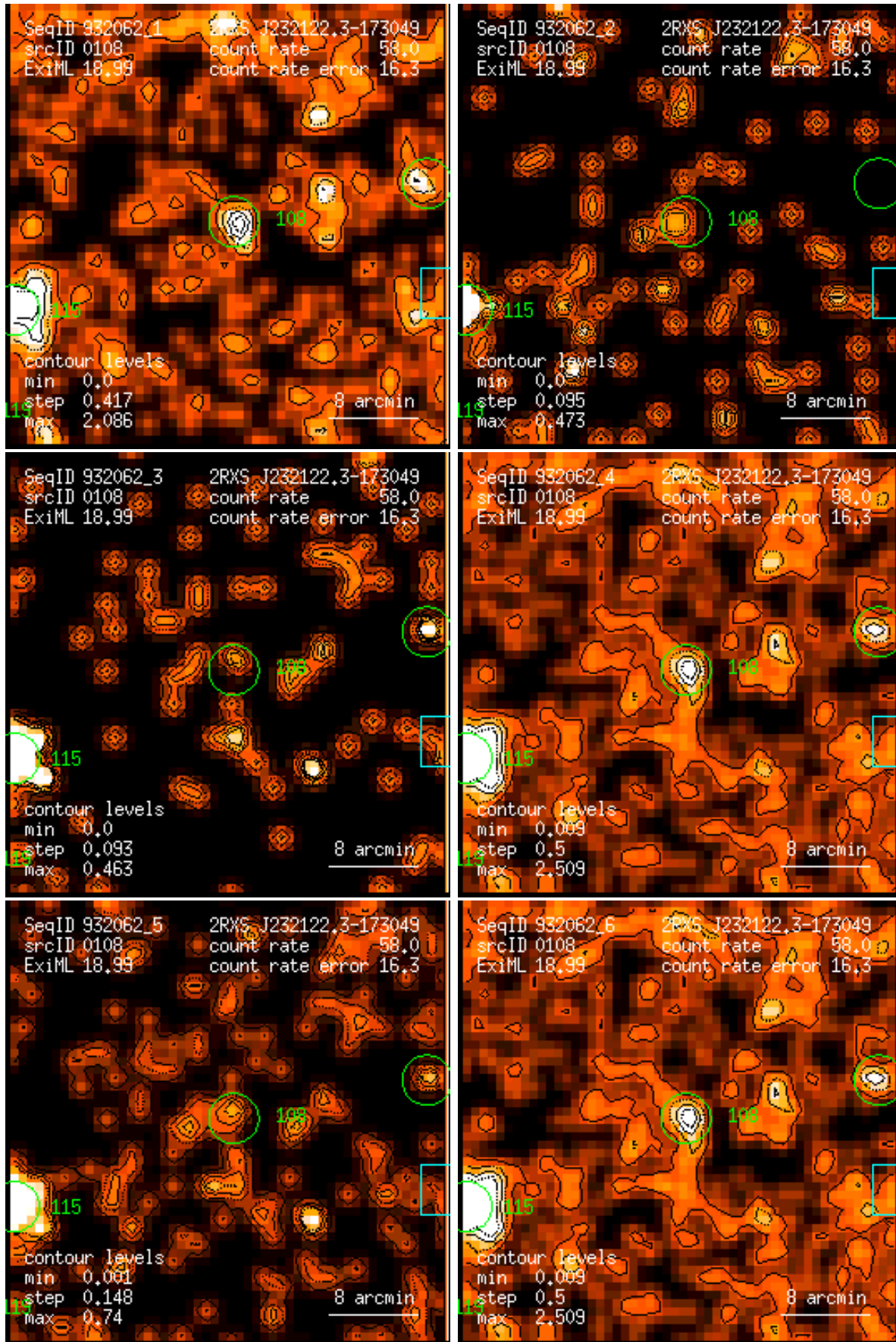
Figure 108: RASS 932062: detection 0108: band rate images, Gaussian filter: (1) PSPC channels 11 – 41, (2) 52 – 90, (3) 91 – 201, (4) 11 – 235, (5) 52 – 201, (6) 11 – 201. Broad band rates in counts/ks. Band rate contour levels in counts/ks/arcmin 2 .
