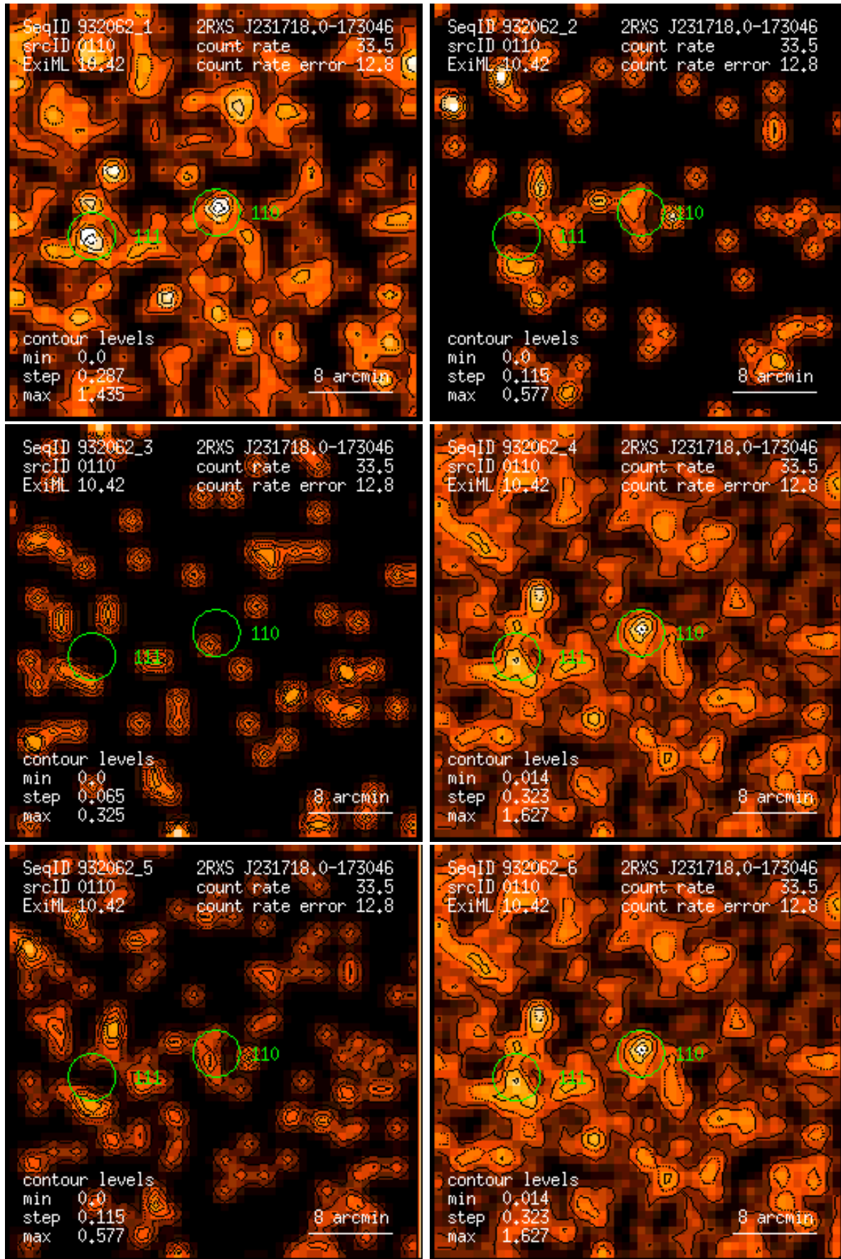
Figure 110: RASS 932062: detection 0110: band rate images, Gaussian filter: (1) PSPC channels 11 – 41, (2) 52 – 90, (3) 91 – 201, (4) 11 – 235, (5) 52 – 201, (6) 11 – 201. Broad band rates in counts/ks. Band rate contour levels in counts/ks/arcmin 2 .
